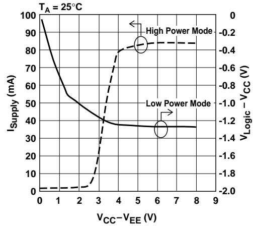
Figure 5. Typical Supply Current & V_{Loic} vs. Supply Voltage.
