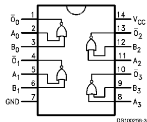
Pin Assignment for DIP and Flatpak
