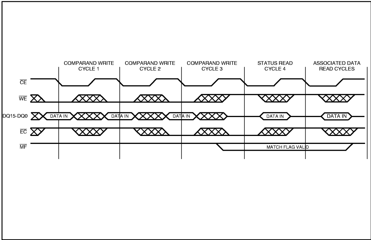
Figure 16. Cycle-to-Cycle Timing
