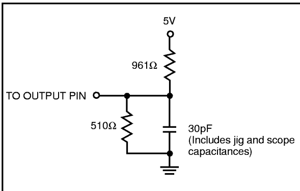
Figure 7. Test Load A
