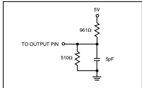
Figure 8. Test Load B
