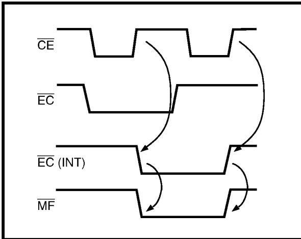
Figure 4. \overline{EC} Internal Timing Diagram
