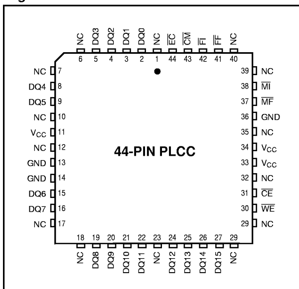
Figure 2. Pinout for QS761480
