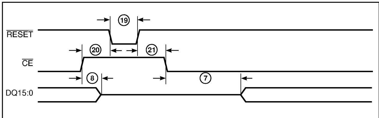
Figure 10. Reset Timing
