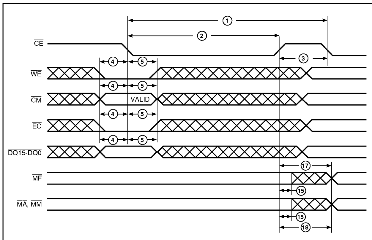
Figure 13. Match-Cycle Timing: Stand-Alone Mode
