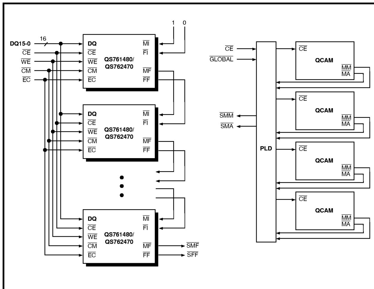
Figure 5. Depth Cascaded QCAMs
