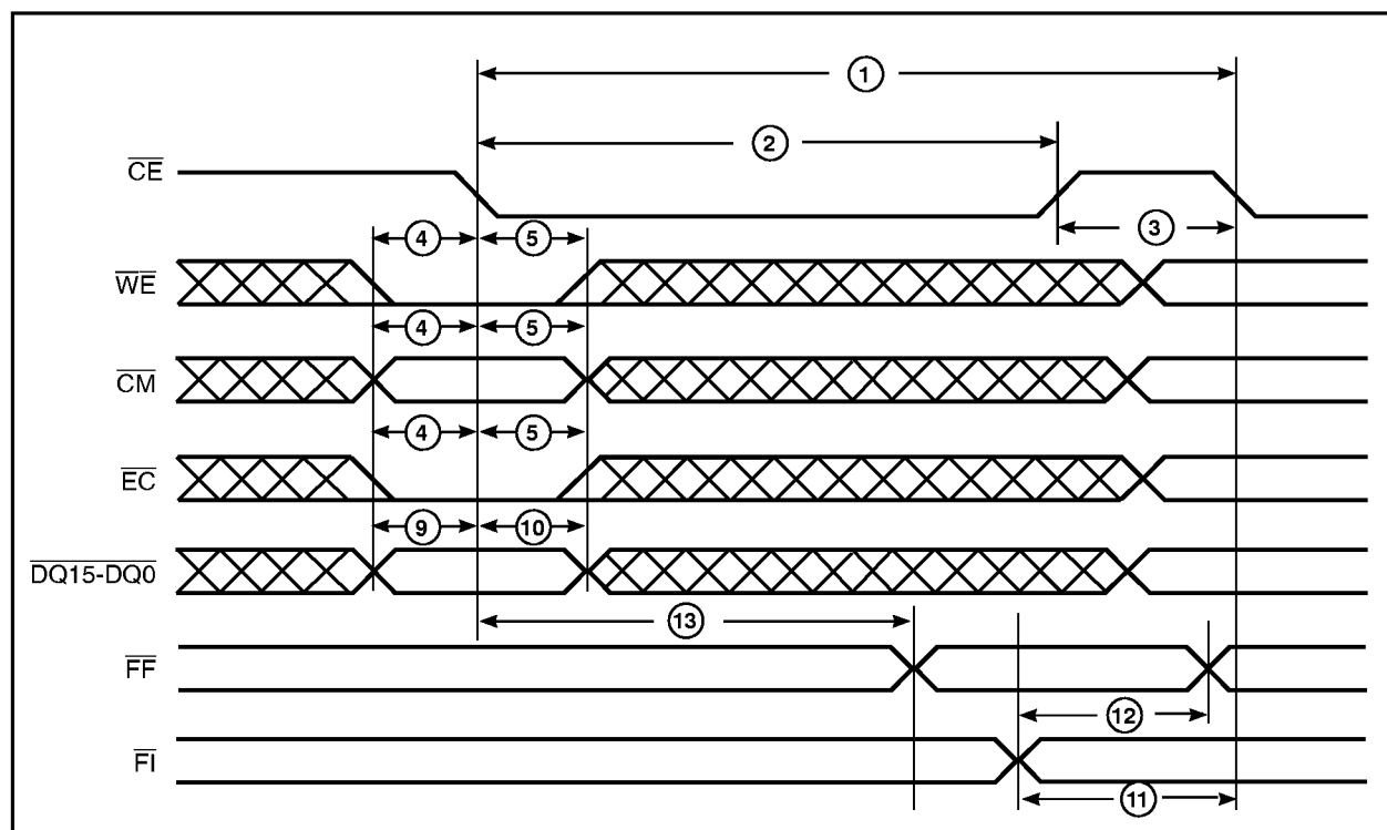
Figure 12. Write Cycle Timing
