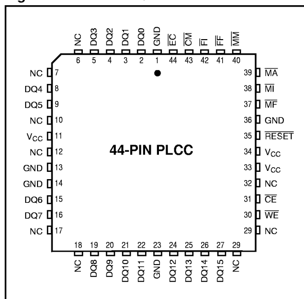
Figure 3. Pinout for QS762470
