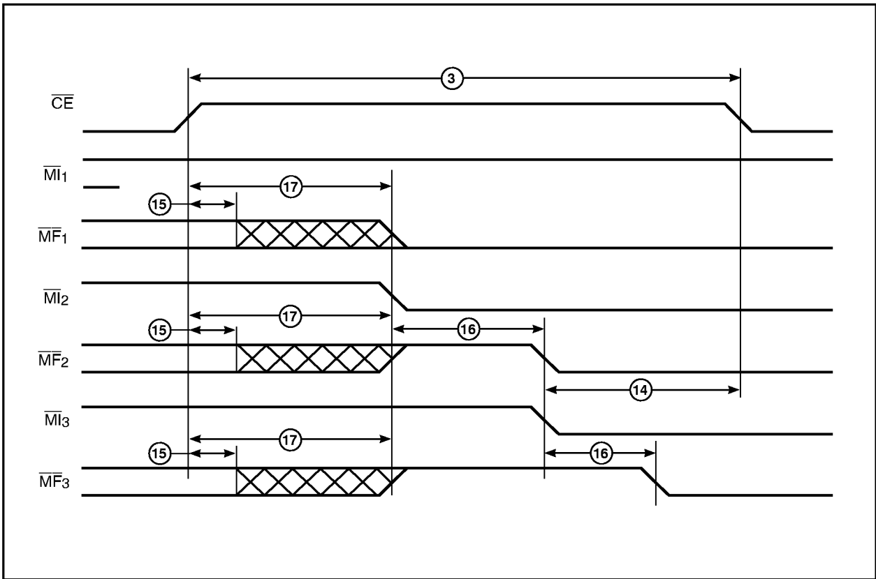
Figure 14. Match Cycle Timing: 3 Daisy-Chained QCAMS, Match in QCAM 1 Only
