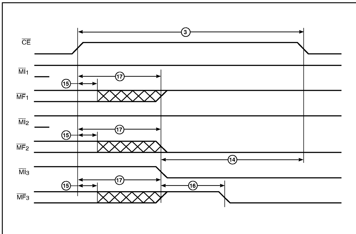
Figure 15. Match Cycle Timing: 3 Daisy-Chained QCAMS, Match in QCAM 2 Only
