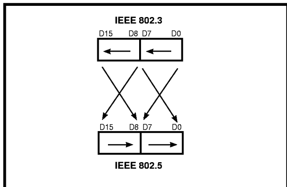
Figure 6. Bit Mapping Between IEEE 802.3 and IEEE 802.5
