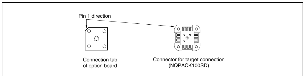
Figure 3-9. Pin 1 Direction Marking of Connector (Top View)
