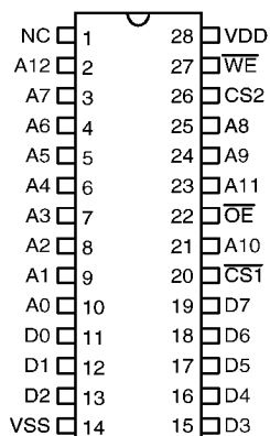
HT6264-70 - 28 DIP/SDIP/SOP
