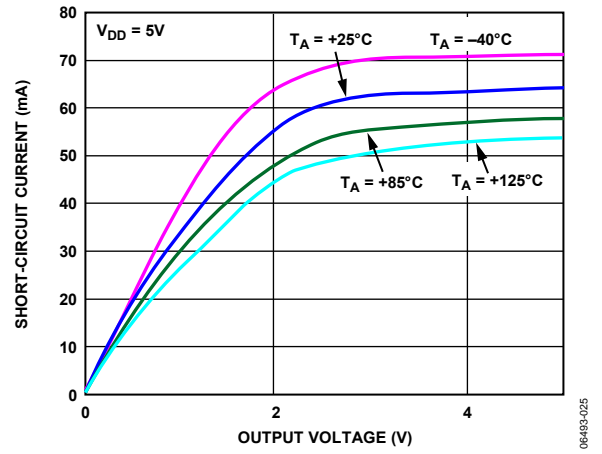
Figure 26. Output Short-Circuit Current
