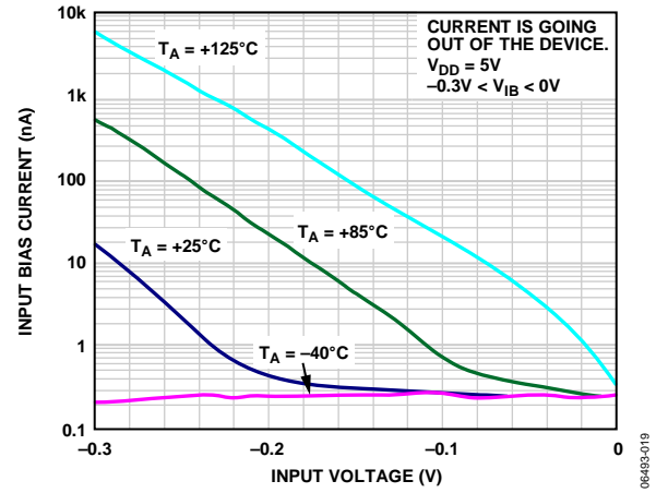
Figure 20. Below Ground Input Bias Current
