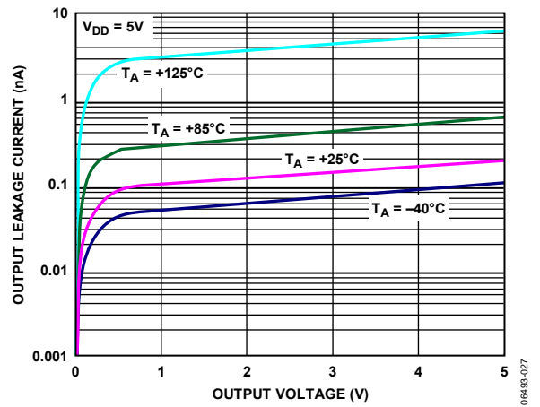
Figure 27. Output Leakage Current
