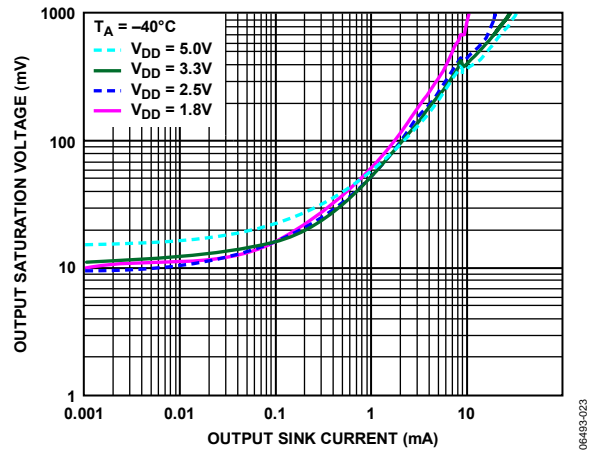
Figure 25. Output Saturation Voltage vs. Output Sink Current
