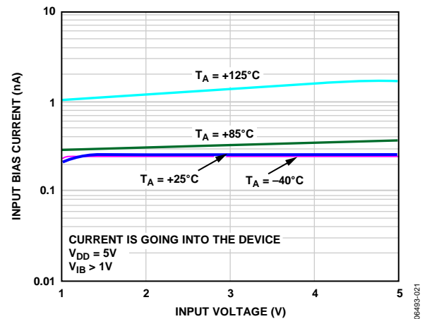
Figure 21. High Level Input Bias Current
