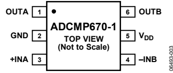
Figure 3. Pin Configuration
