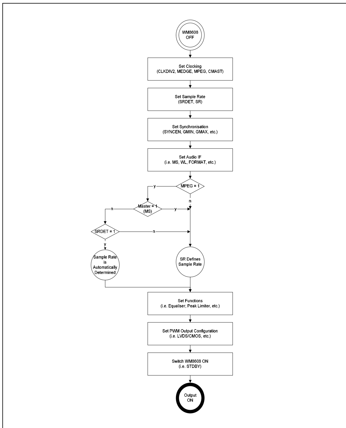
Figure 37 WM8608 Start-up
