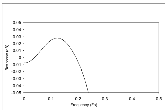
Figure 30 Digital filter Ripple – 176.4kHz and 192kHz
