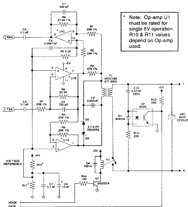
FIGURE 2: Single 5V Hybrid Version
