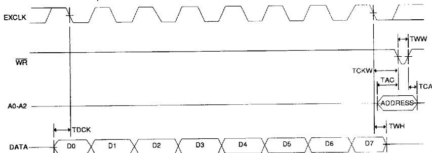
WRITE TIMING DIAGRAM (SERIAL VERSION)
