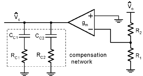
FIGURE 3. Compensation Network
