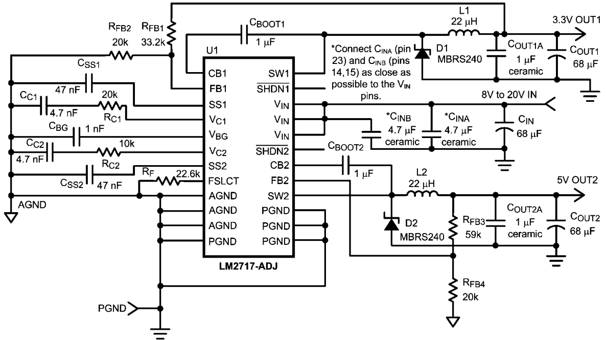
FIGURE 5. 5V, 3.3V Output Application
