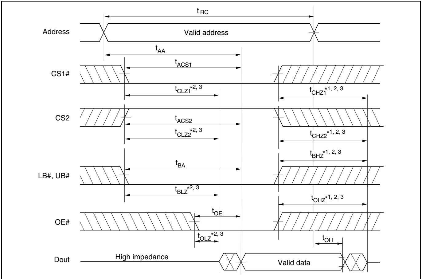
Read Timing Waveform (WE# = V IH )
