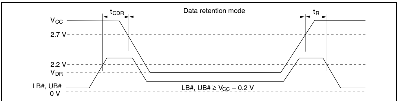
Low V_{CC} Data Retention Timing Waveform (3) (LB#, UB# Controlled)
