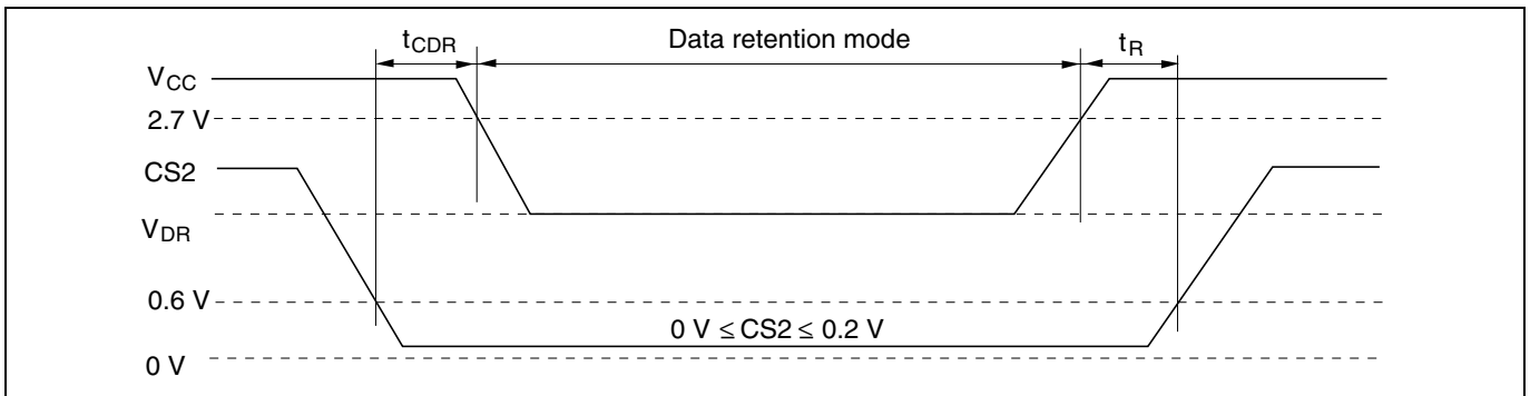
Low V_{CC} Data Retention Timing Waveform (2) (CS2 Controlled)
