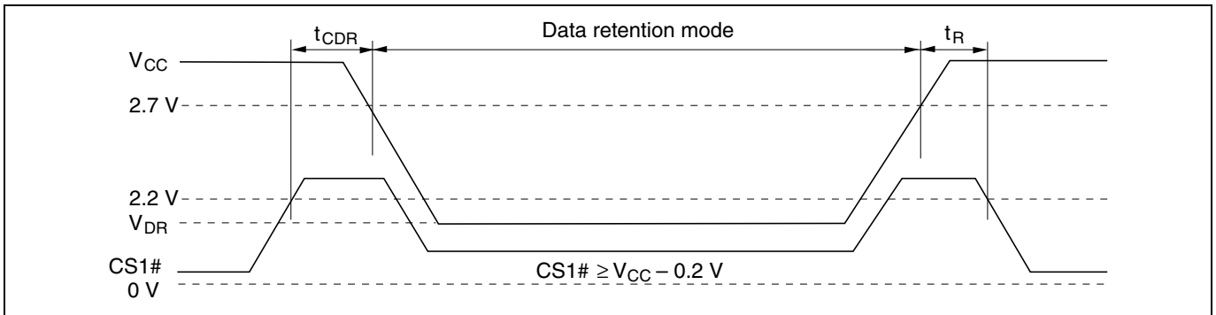
Low V_{CC} Data Retention Timing Waveform (1) (CS1# Controlled)
