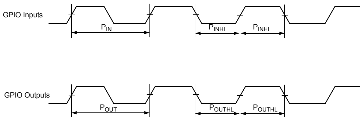
Figure 4-34 GPIO Timing
