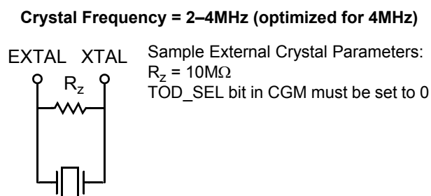
Figure 4-6 Crystal Oscillator
