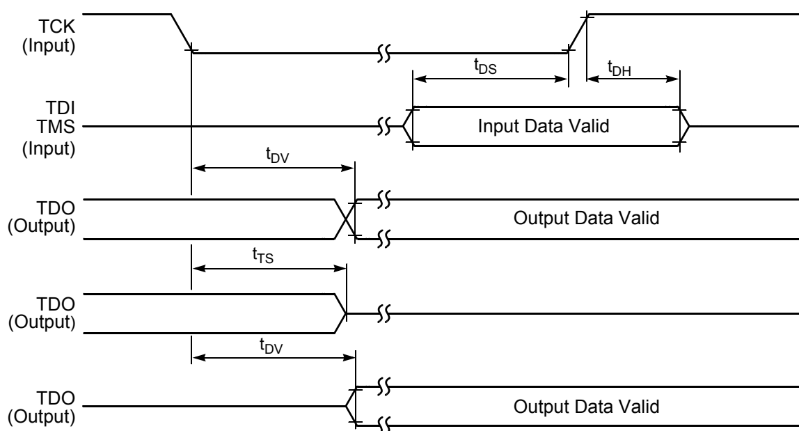
Figure 4-31 Test Access Port Timing Diagram
