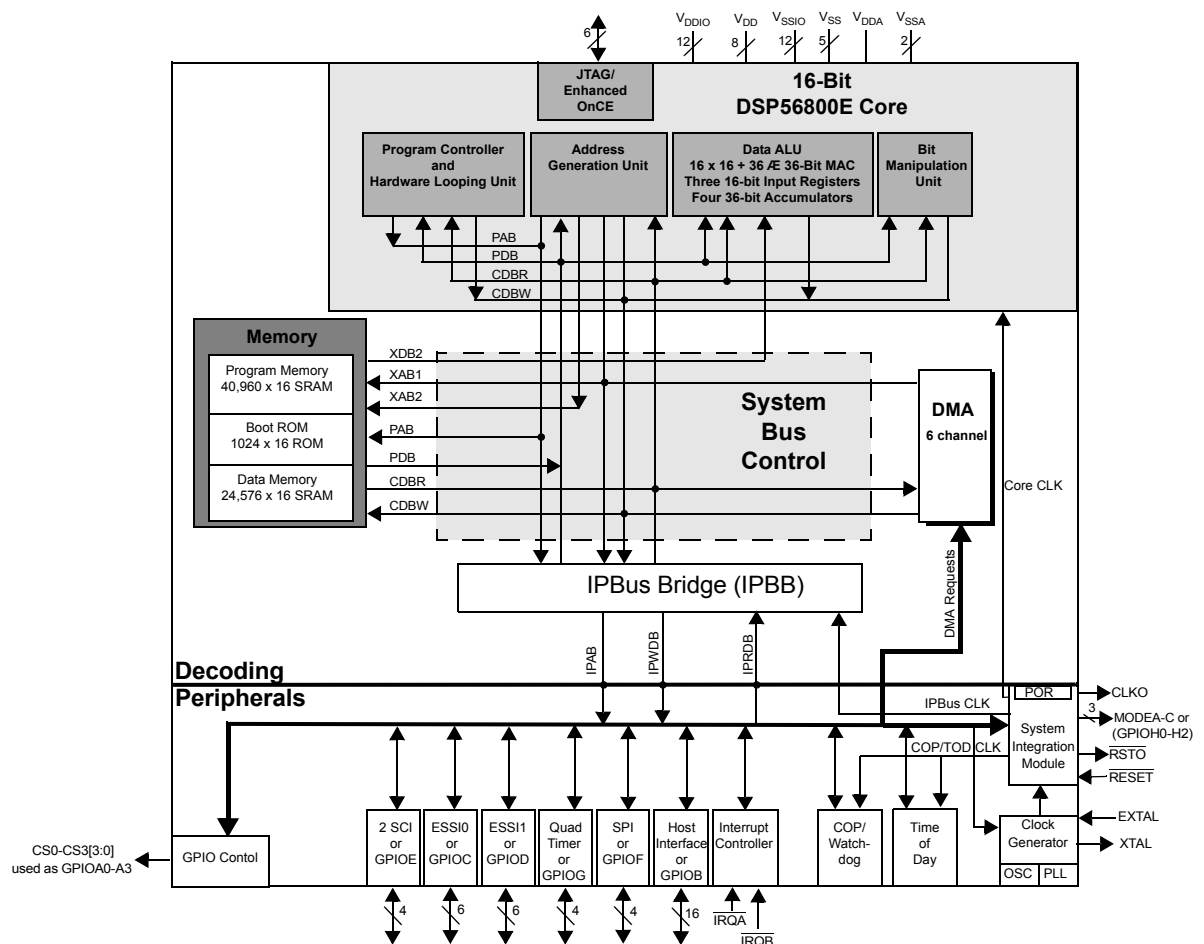
56857 Block Diagram
