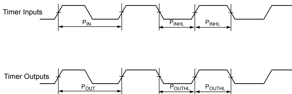
Figure 4-25 Timer Timing
