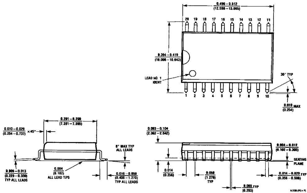
Small Outline Package (M) Order Number DM74AS804BWM NS Package Number M20B
