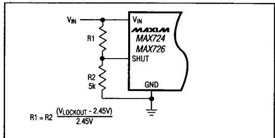
Figure 7. Undervoltage Lockout Application
