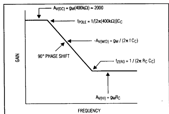
Figure 5. Error-Amplifier Gain as Set by R_C and C_C at V_C Pin
