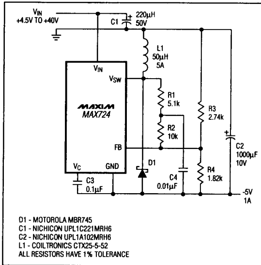
Figure 8. Positive-to-Negative DC-DC Inverter
