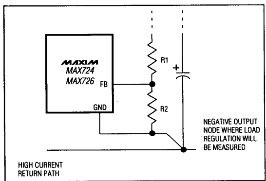
Figure 4. Recommended Ground Connection
