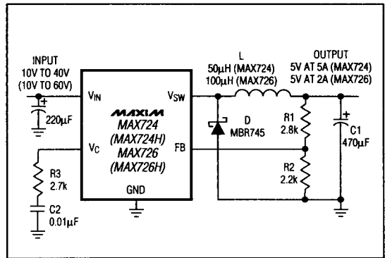
Figure 2. Basic Step-Down Converter
