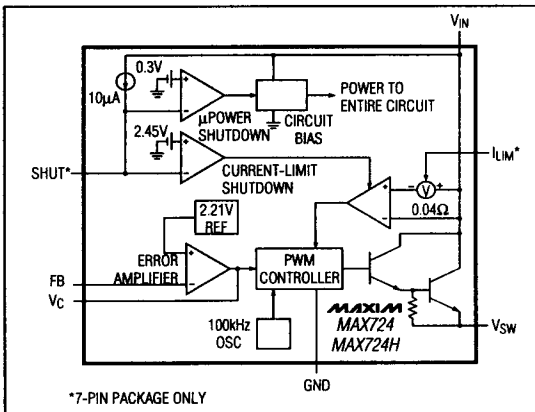
Figure 1. MAX724 Block Diagram
