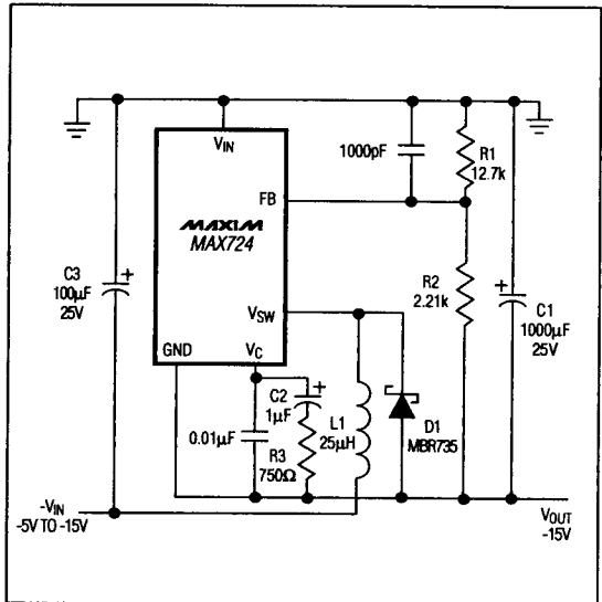
Figure 9. Negative Step-Up DC-DC Converter
