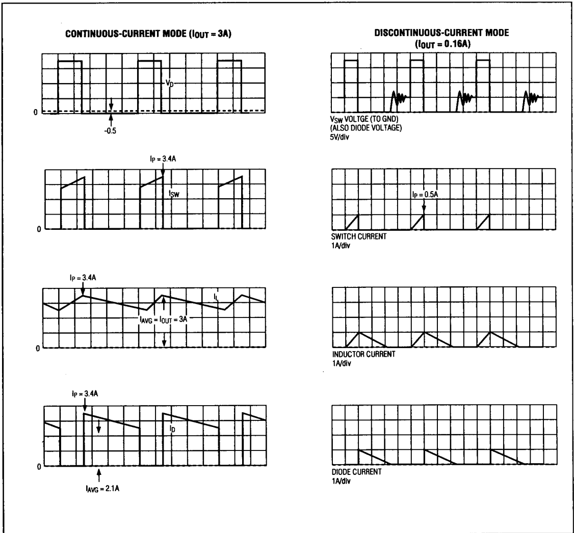
Figure 3. MAX724 Step-Down Converter Waveforms with V_{IN} = 20V , L = 50\mu H (all waveforms 2\mu s/div )
