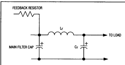
Figure 6. Optional LC Output Filter
