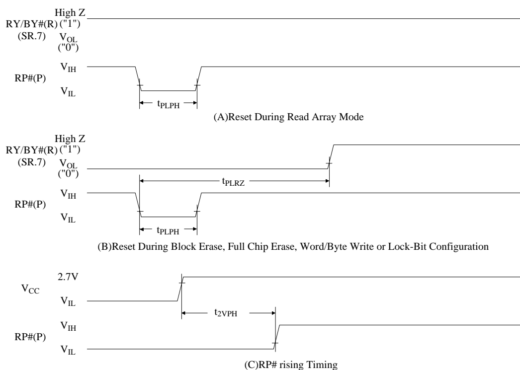
Figure 18. AC Waveform for Reset Operation
