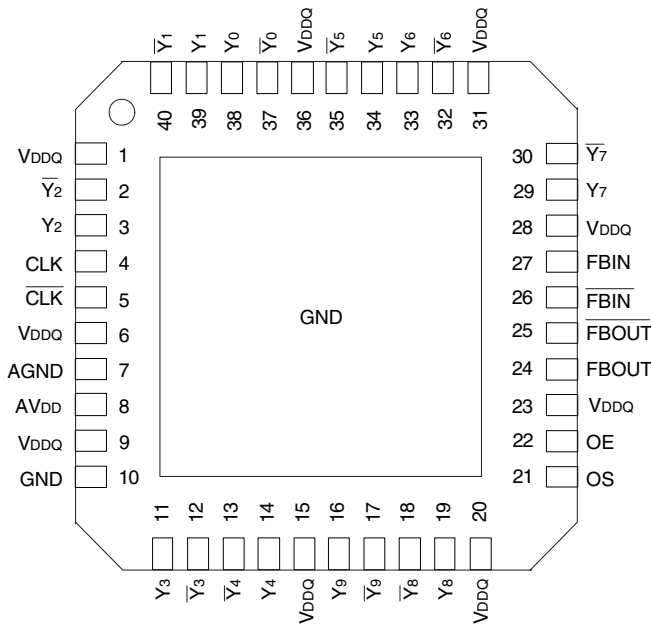
VFOFPN TOP VIEW
