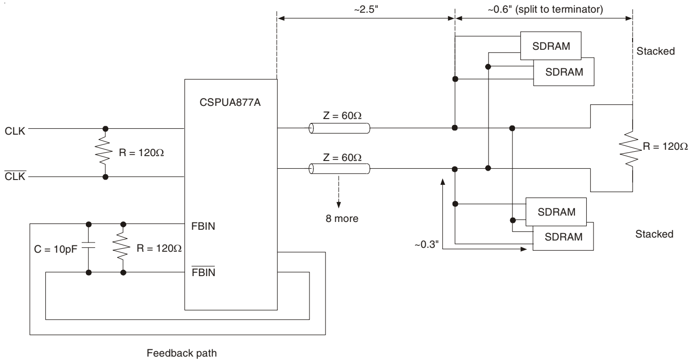
Clock Structure 2
