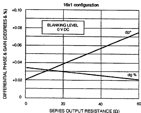
Fig. 9 Phase and Gain vs Resistance
