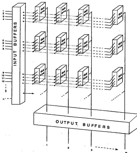
Fig.12 Multi-chip Connections
