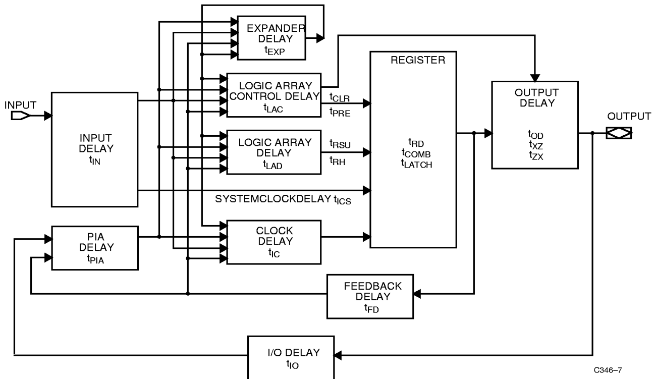
Figure 1. CY7C346/CY7C346B Internal Timing Model
