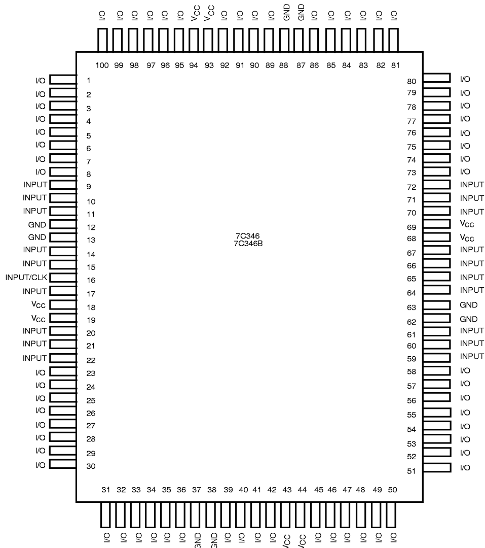
PQFP Top View
