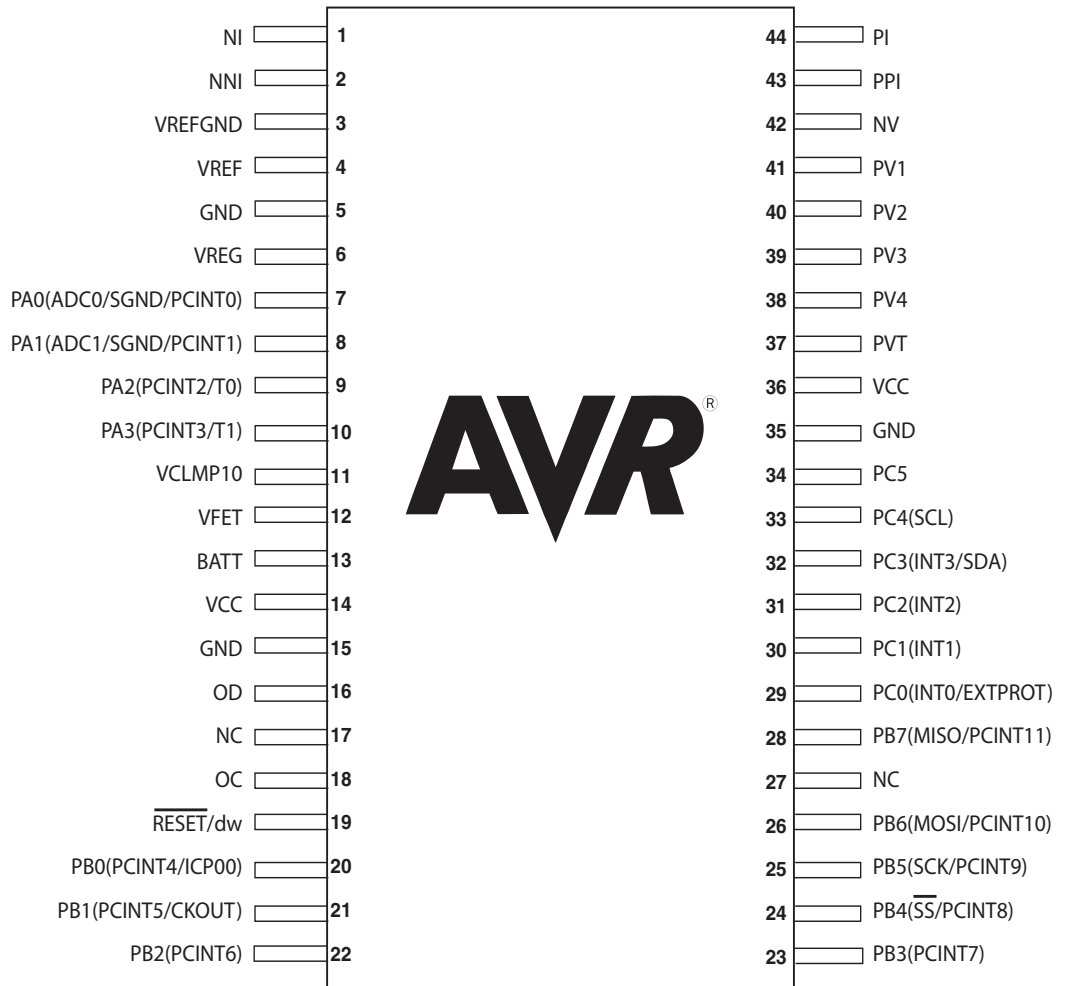
Figure 1-1. TSSOP - pinout ATmega16HVB/32HVB
