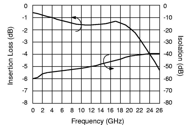
Insertion Loss and Isolation vs. Frequency
