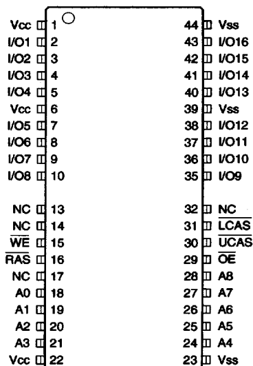
40/44-pin TSOP TYPE ( II ) (400mil) P44/40TP-3B P44/40TP-3B-L
