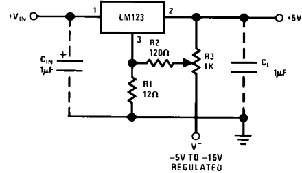
Trimming Output to 5V
