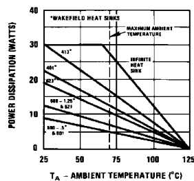
Maximum Average Power Dissipation for LM323A, LM323
