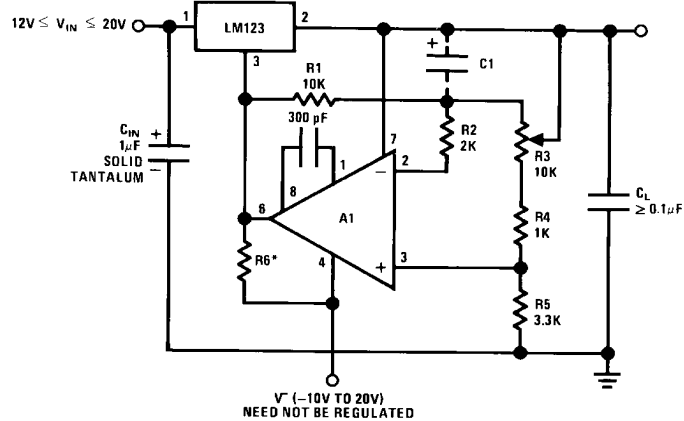
Adjustable Regulator 0V–10V @ 3A
