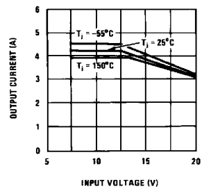
Peak Available Output Current
