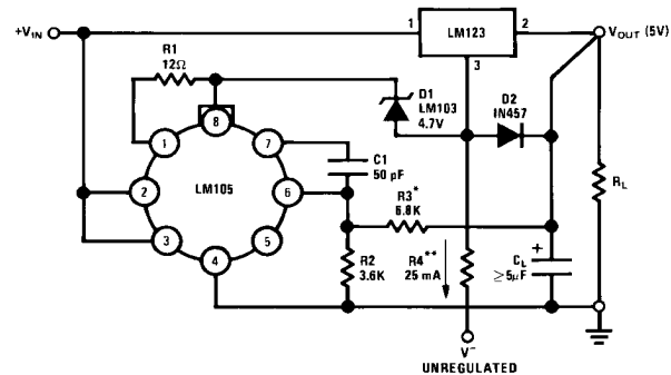
Adjustable Output 5V–10V 0.1% Regulation
