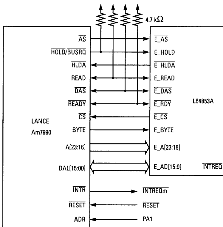
Figure 8.5 L64853A to Am7990 LANCE Interface
