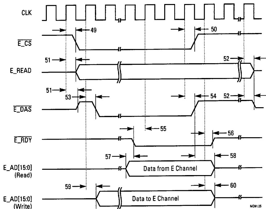
Figure 7.10 E-Channel Register Access Timing
