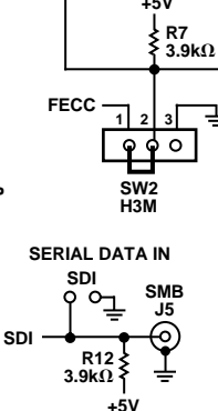
Figure 39. Electrical Schematic of AD9853-xxPCB Evaluation Board
