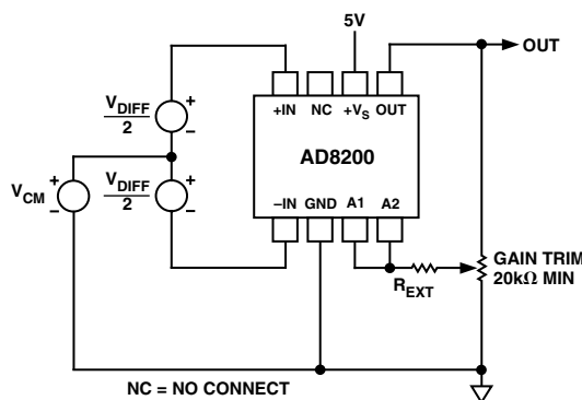
Figure 7. Incremental Gain Trim
