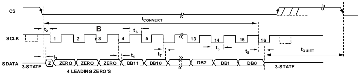
Figure 14. AD7466 Serial Interface Timing Diagram
