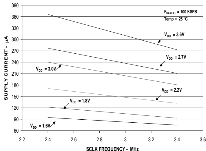
Figure 11. Supply current vs SCLK frequency for a fixed throughput rate and different supply voltages
