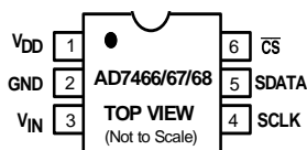
6-Lead SOT-23
