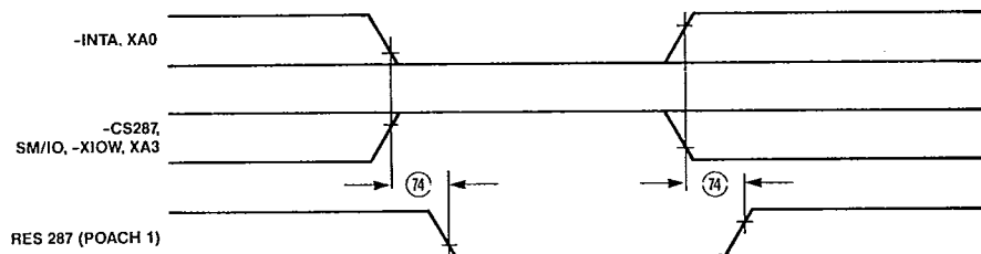
Figure 25. RES 287 Timing
