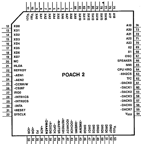
Pin Diagram POACH 2
