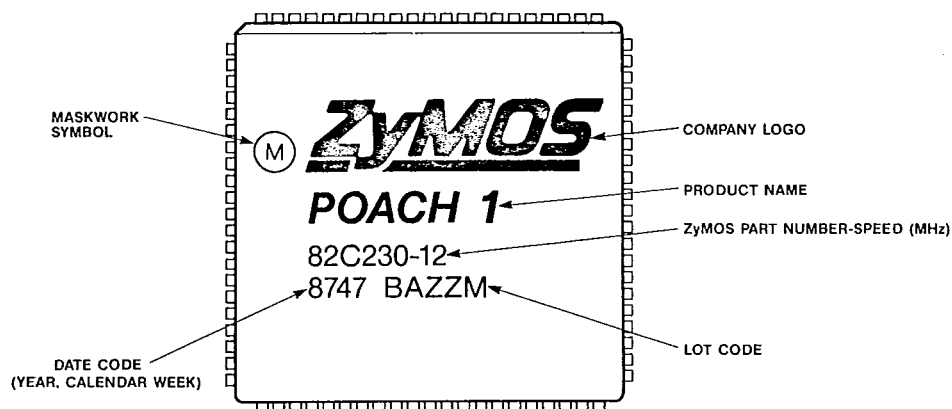
MARKING DETAILS
