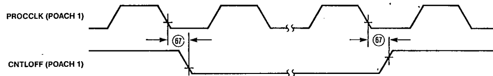
Figure 20. CNTLOFF Timing
