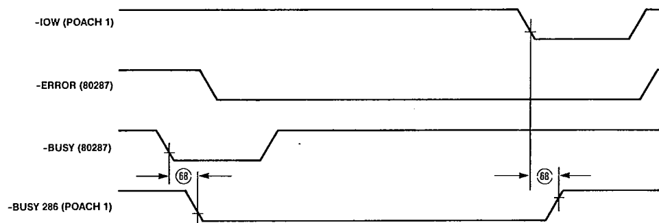
Figure 21. -BUSY286 Timing
