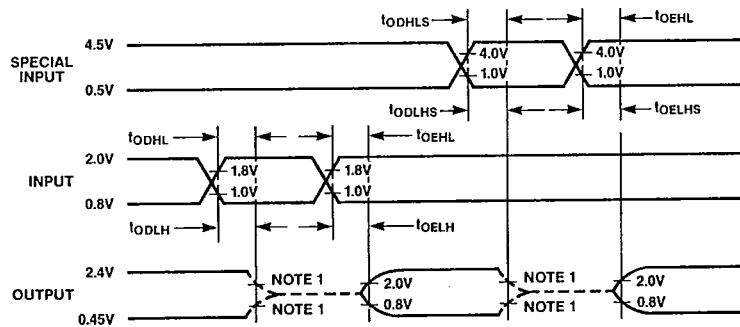
Figure 1C. Output Enable/Disable Time Measurement
