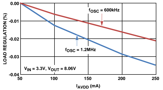
FIGURE 2. I AVDD LOAD REGULATION vs I AVDD
