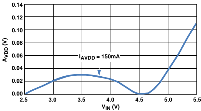
FIGURE 3. I AVDD LINE REGULATION vs V IN
