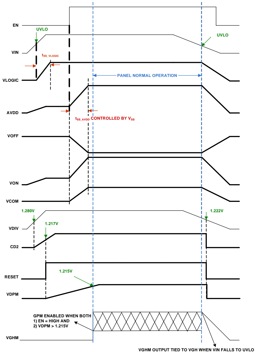
FIGURE 19. ISL97649A POWER ON/OFF SEQUENCE
