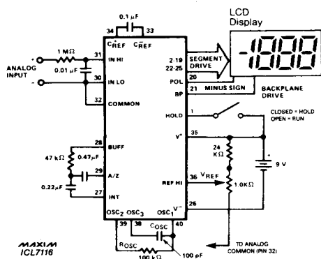
Figure 1. Maxim ICL7116 Typical Operating Circuit, 200mV Reference
