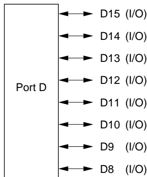
Figure 10B-17 Port D Pin Functions (Modes 4 to 6)
