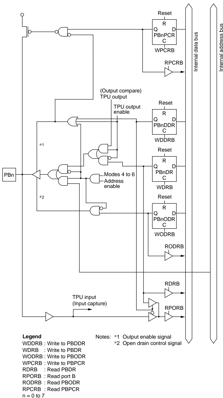
Figure C-19 Port B Block Diagram (Pins PB0 to PB7)
