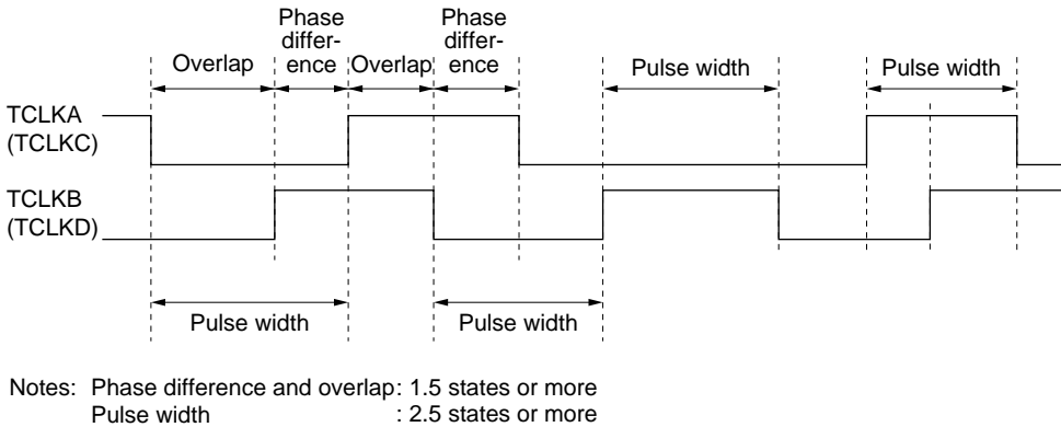
Figure 11-48 Phase Difference, Overlap, and Pulse Width in Phase Counting Mode
