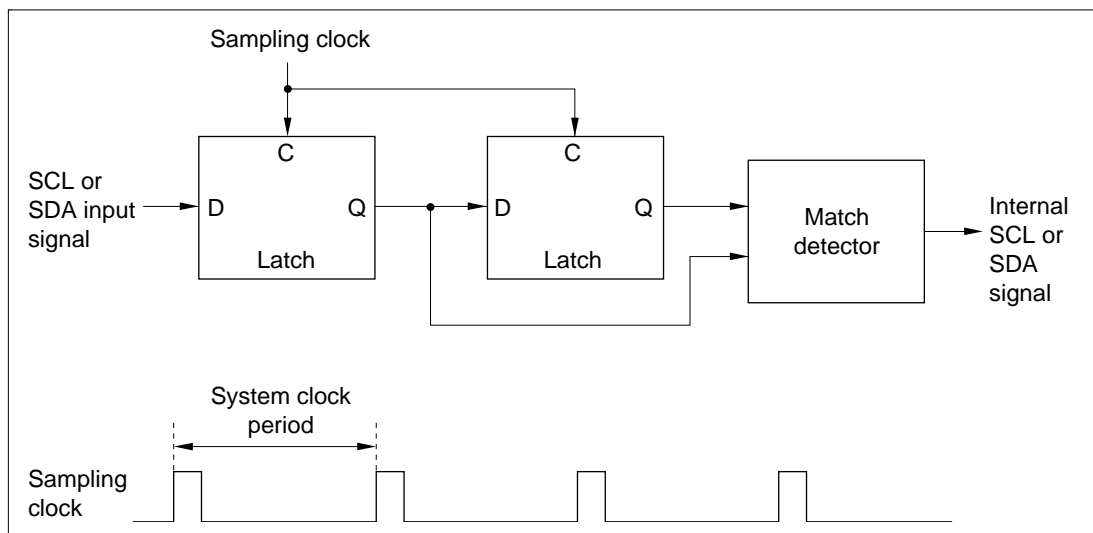
Figure 18-18 Block Diagram of Noise Canceled
