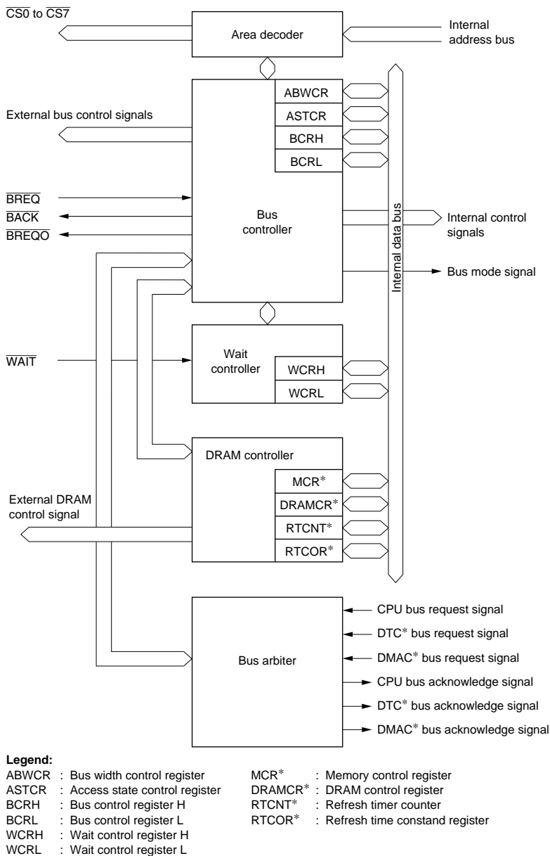
Figure 7-1 Block Diagram of Bus Controller
