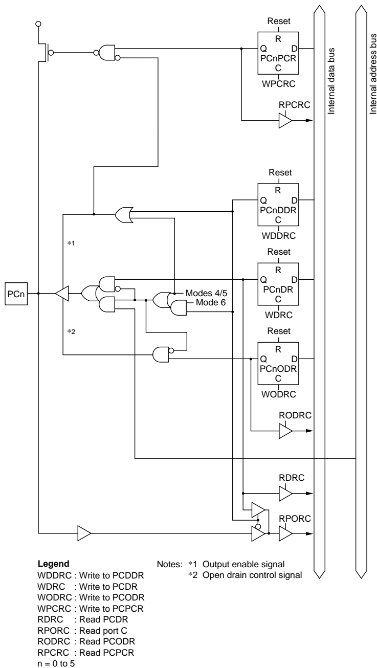
Figure C-20 (a) Port C Block Diagram (Pins PC0 to PC5)
