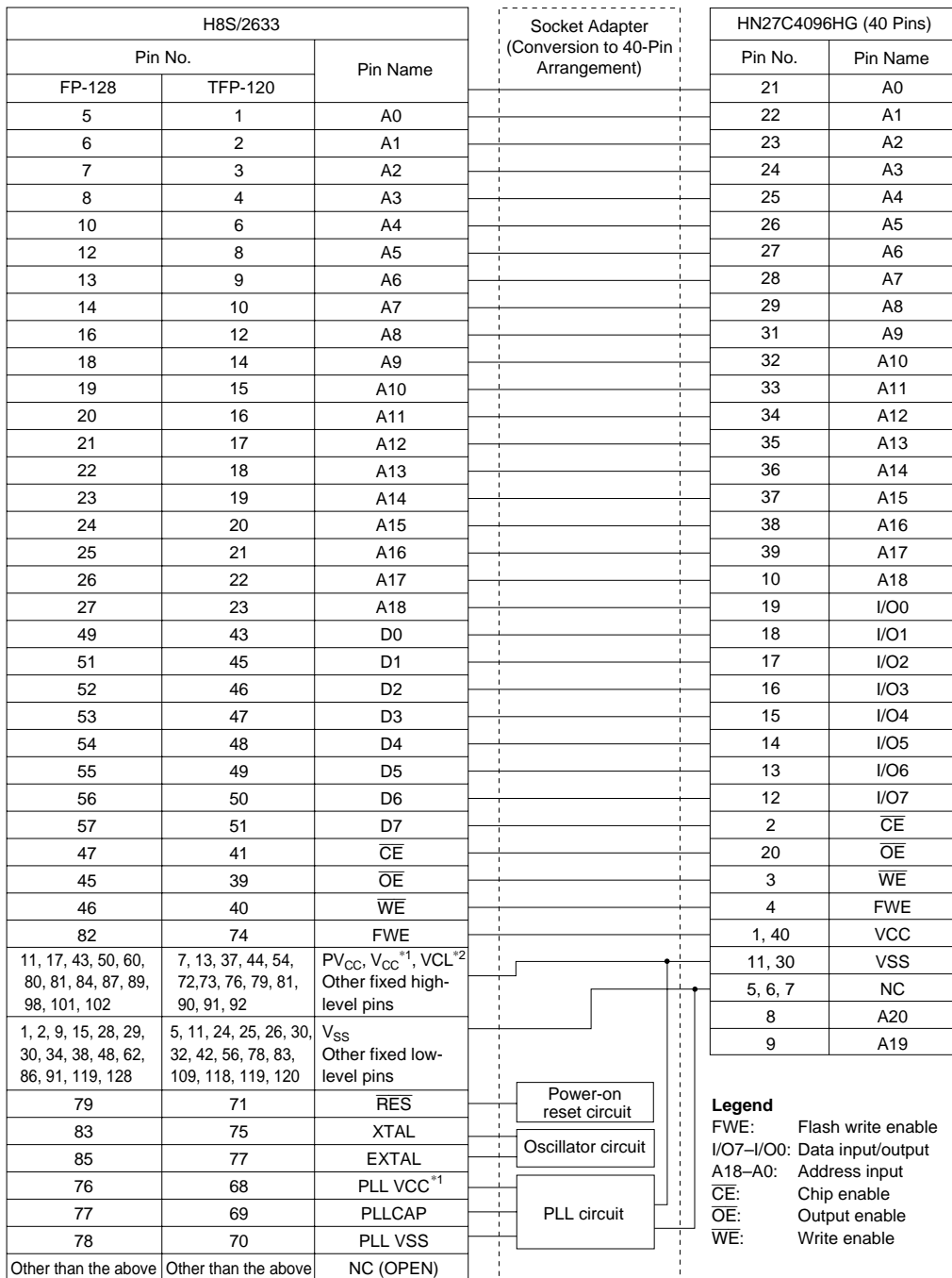
Figure 22-18 Socket Adapter Pin Correspondence Diagram
