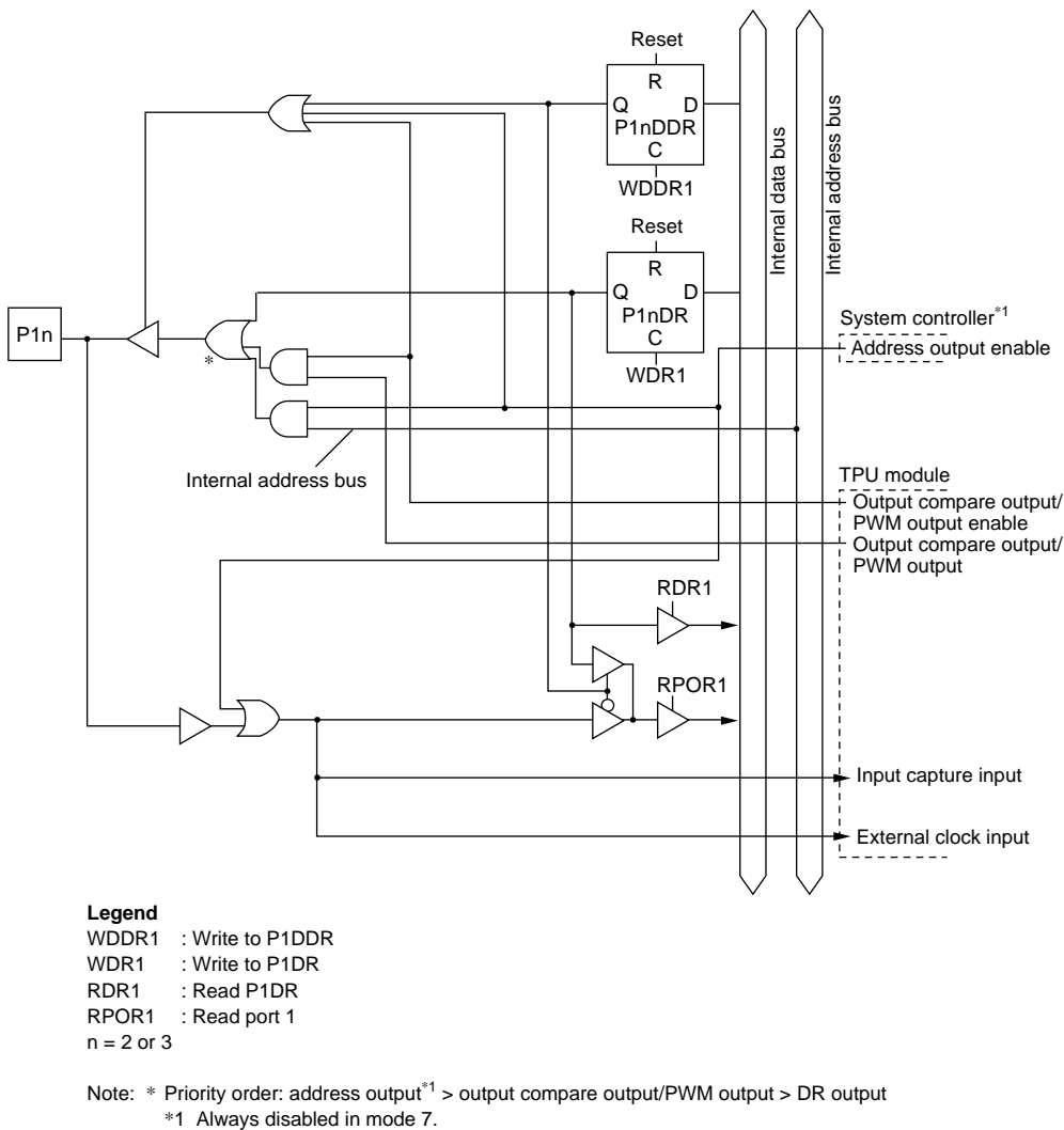
Figure C-13 (b) Port 1 Block Diagram (Pins P12 and P13)
