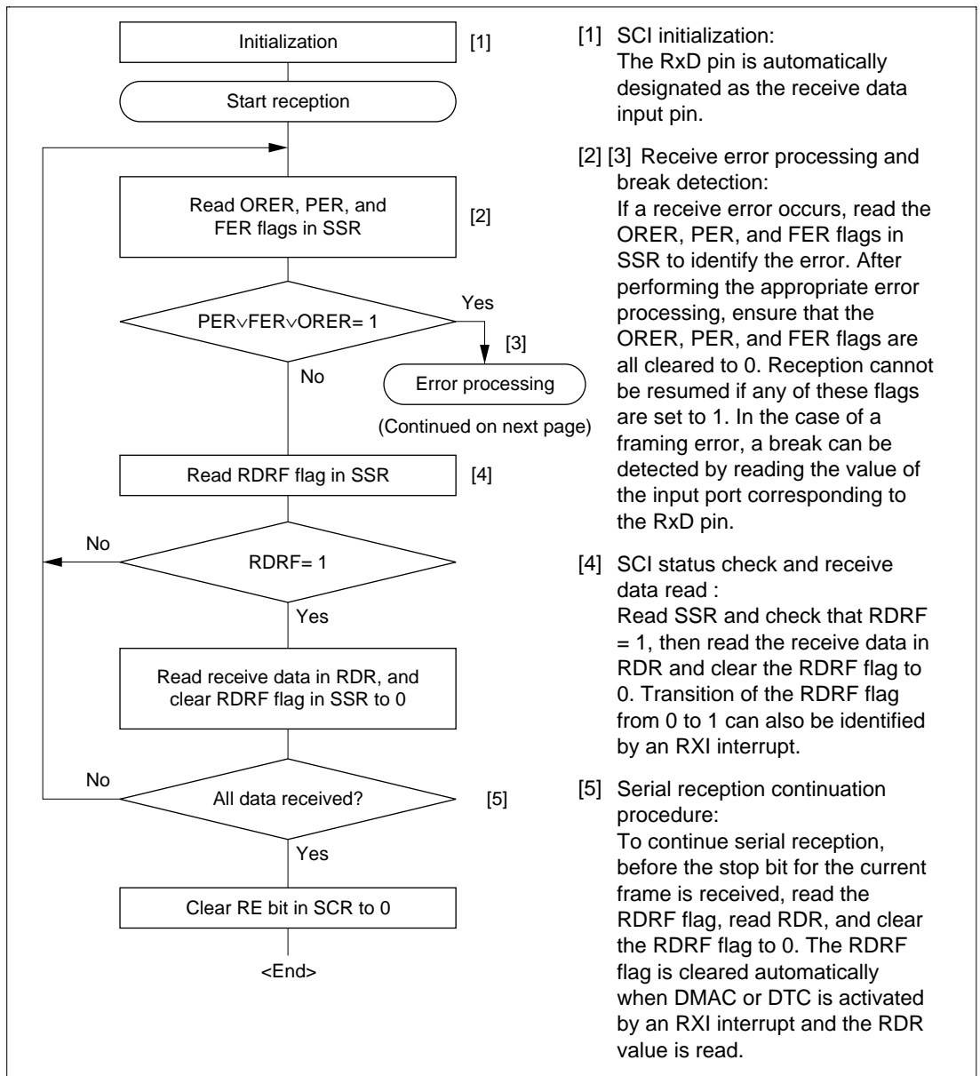
Figure 16-7 Sample Serial Reception Data Flowchart
