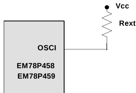
Fig. 21 Circuit for Internal C Oscillator Mode
