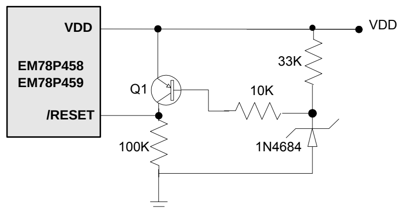
Fig. 23 Circuit 1 for the Residue Voltage Protection
