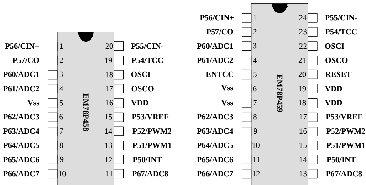
Fig. 1 Pin Assignment
