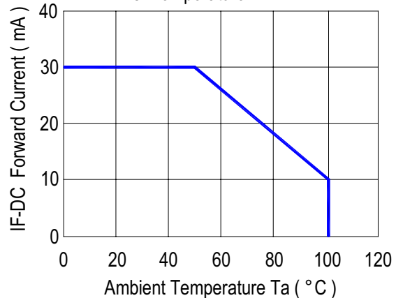
FIG. 6 Maximum Forward Current vs. Temperature
