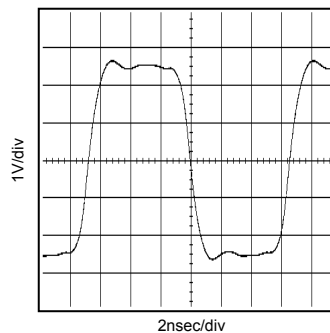
Fig.44 Output Waveform (VDD=5.0V, Select="L", Output=75MHz)
