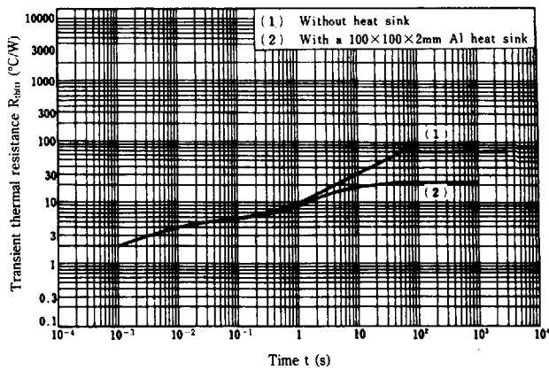
R_{th}(t) - t
