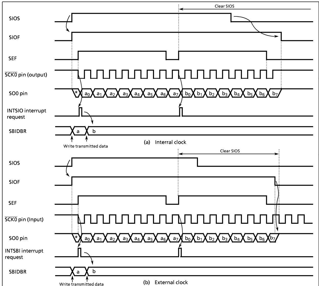
Figure 2-58. Transfer Mode
