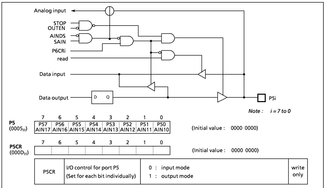
Figure 2-8. Port P5
