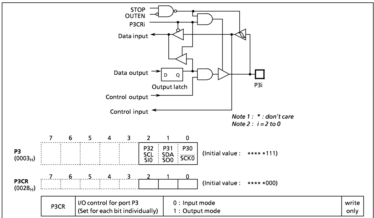
Figure 2-6. Port P3
