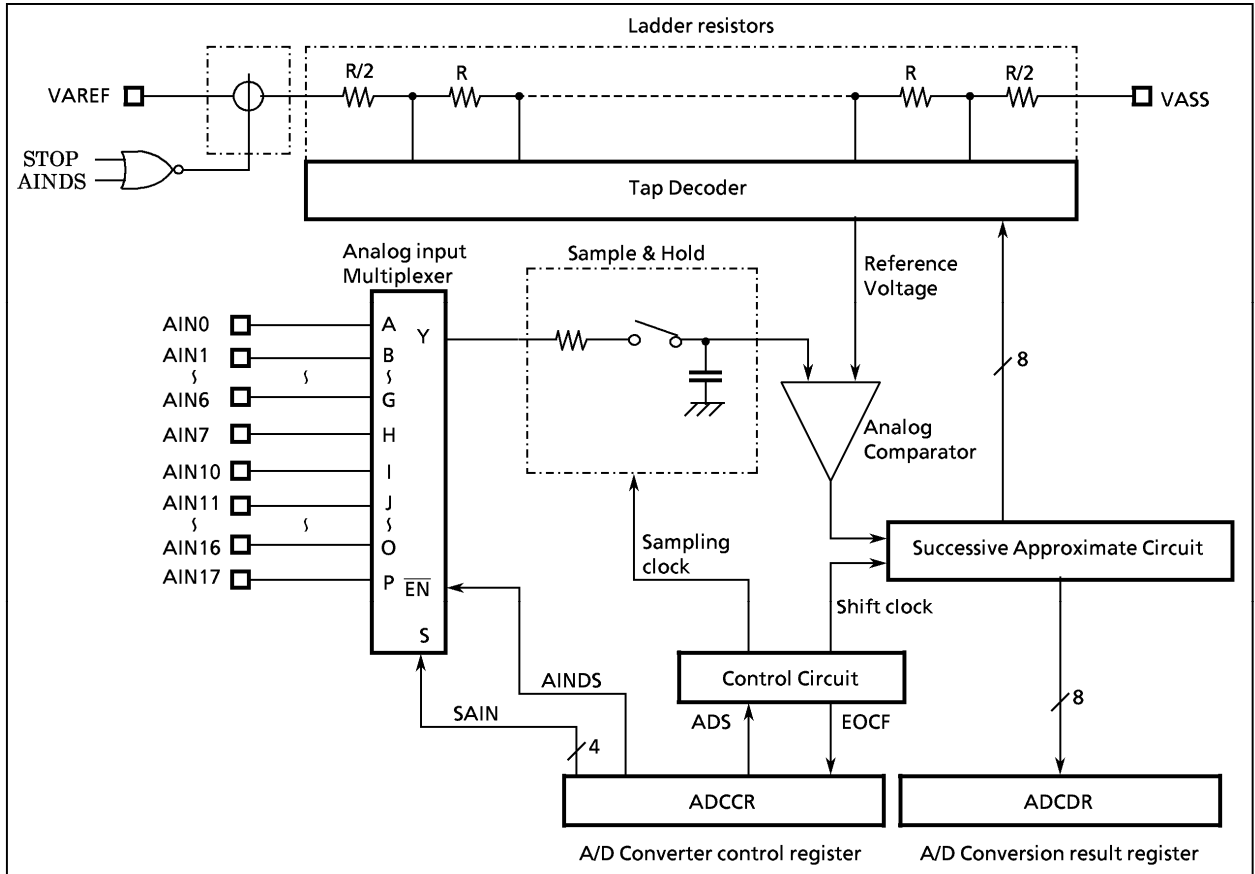
Figure 2-74. A/D Converter
