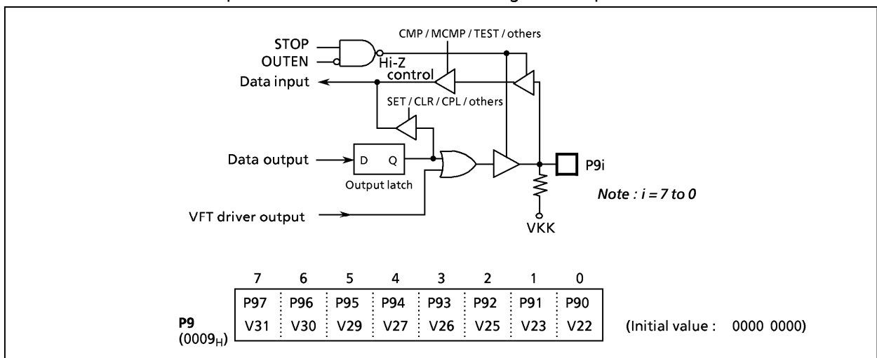
Figure 2-12. Port P9
