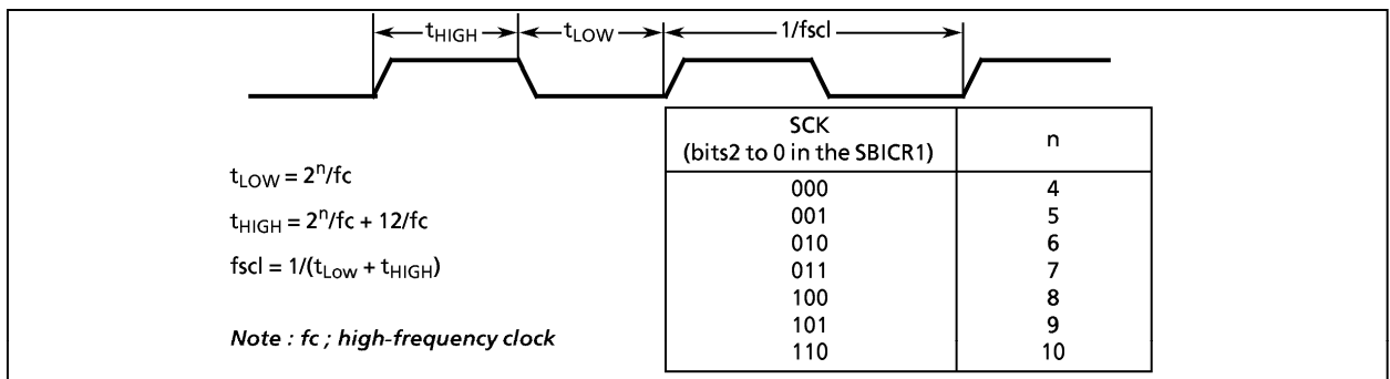
Figure 2-42. Clock Source
