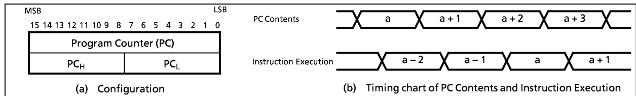
Figure 1-3. Program Counter
