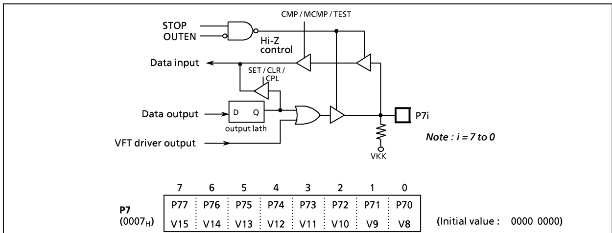
Figure 2-10. P7 Port
