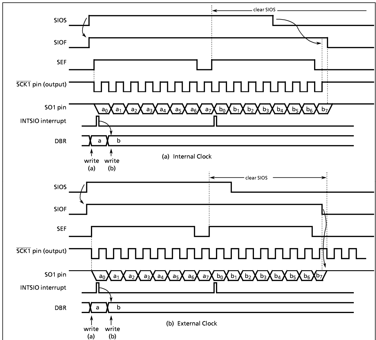
Figure 2-69. Transfer Mode (Example: 8-bit, 1 Word Transfer)
