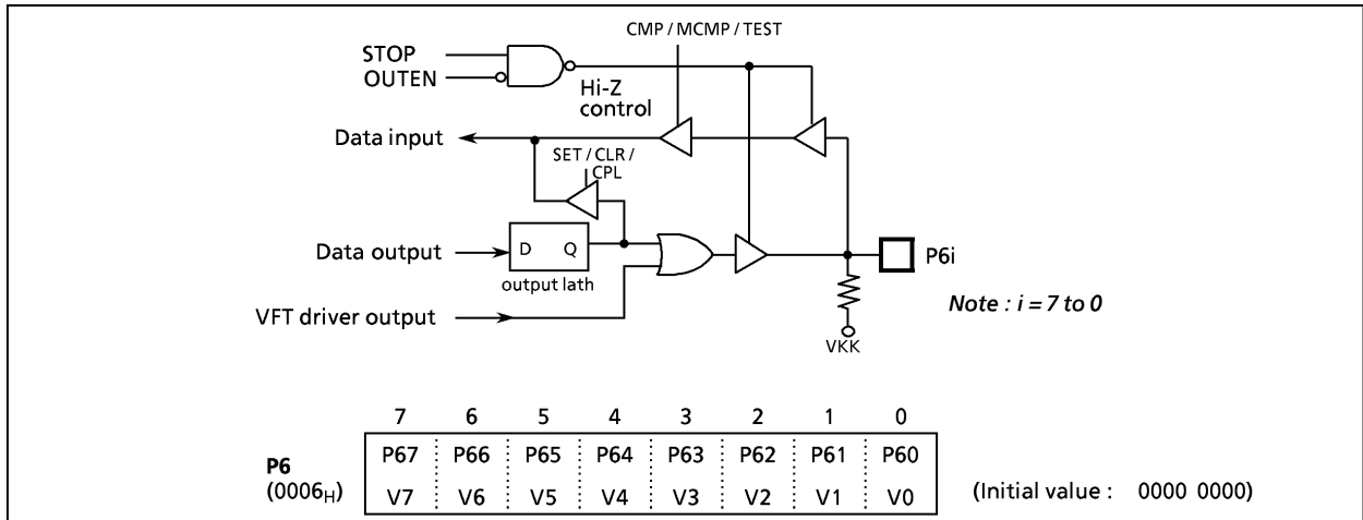
Figure 2-9. P6 Port
