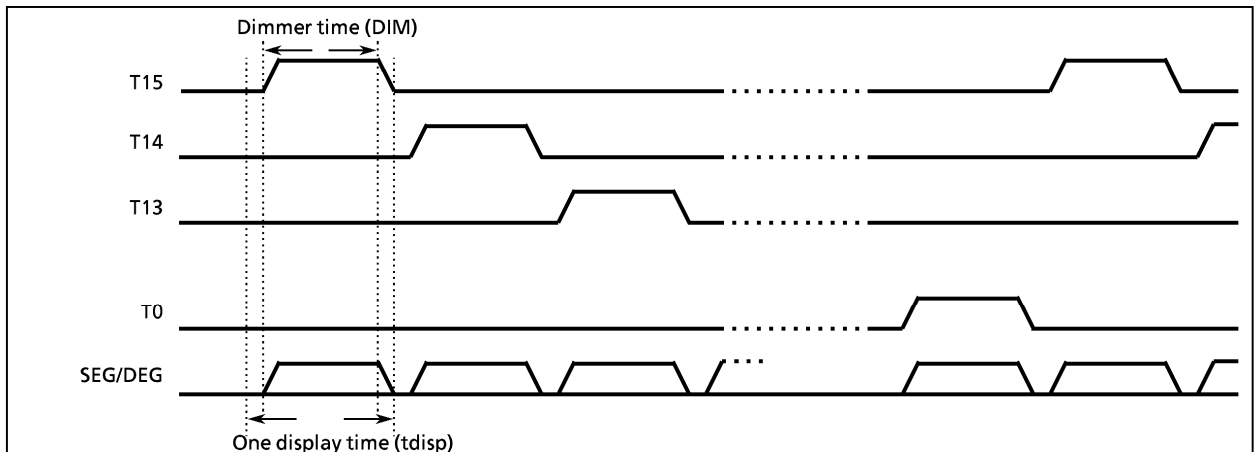
Figure 2-83. VFT Drive Waveform and Display timing
