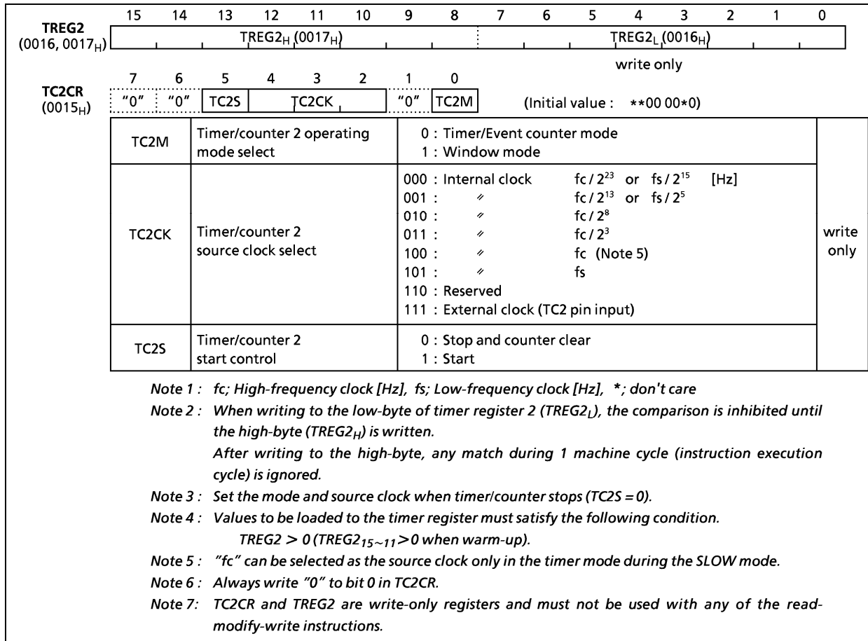
Figure 2-28. Timer Register 2 and TC2 Control Register
