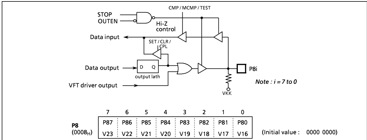
Figure 2-11. P8 Port
