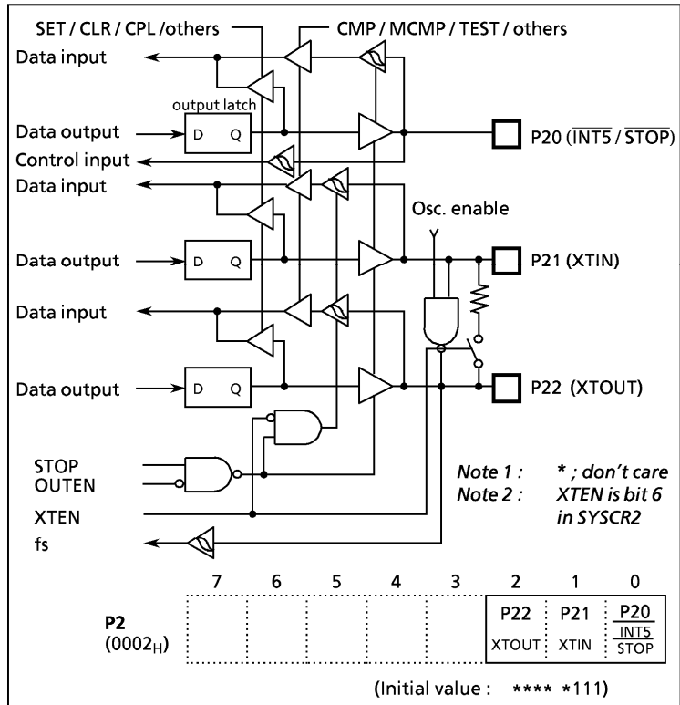
Figure 2-5. Port P2
