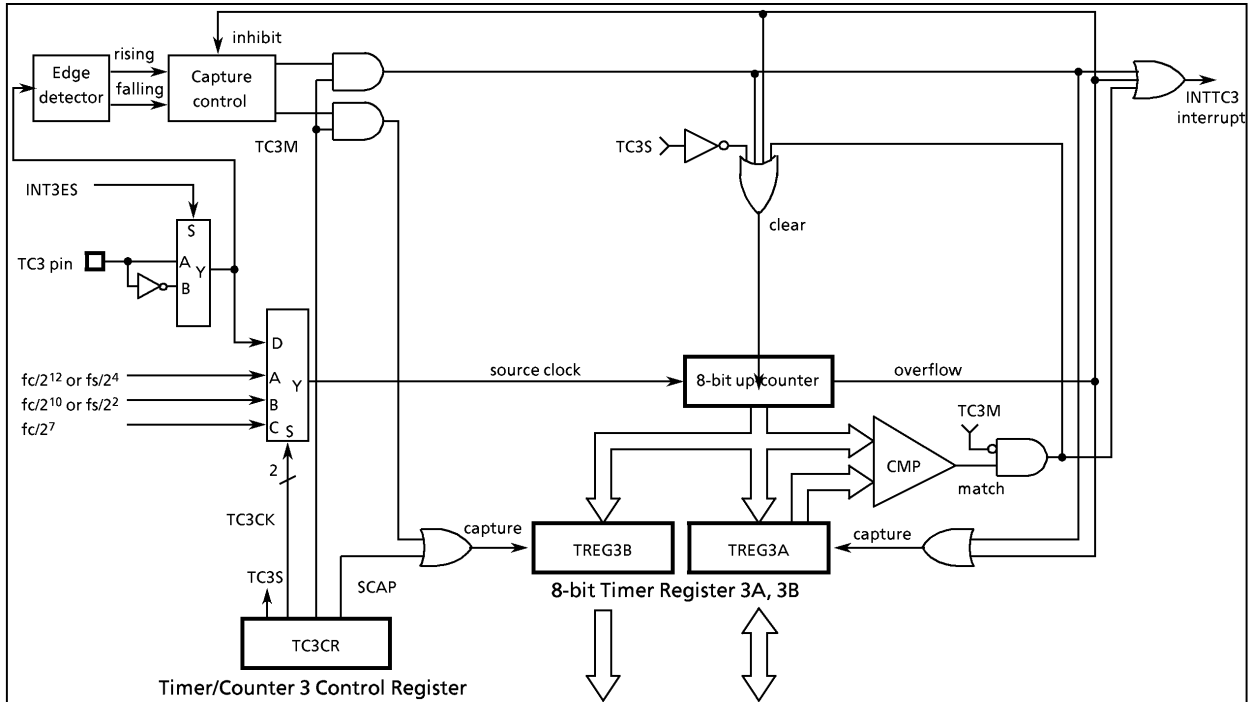
Figure 2-30. Timer/Counter 3
