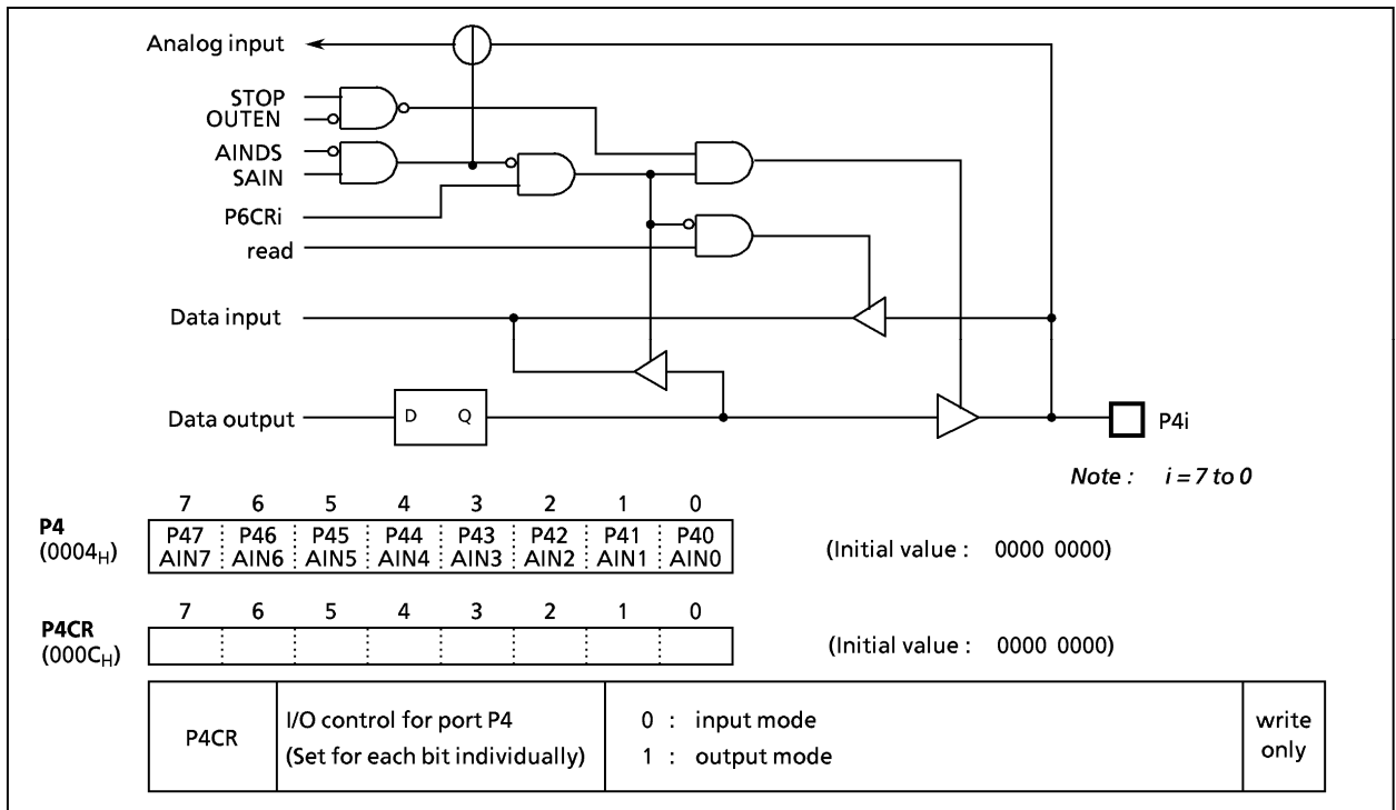
Figure 2-7. Port P4
