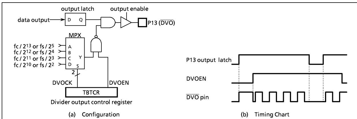
Figure 2-17. Divider Output
