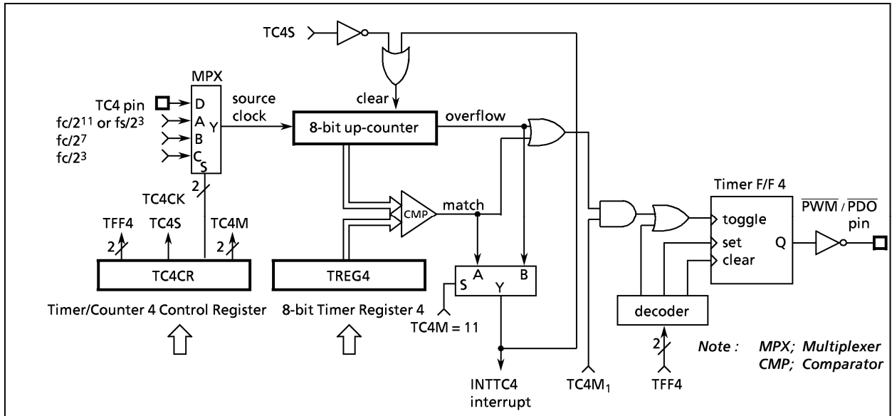
Figure 2-34. Timer/Counter 4
