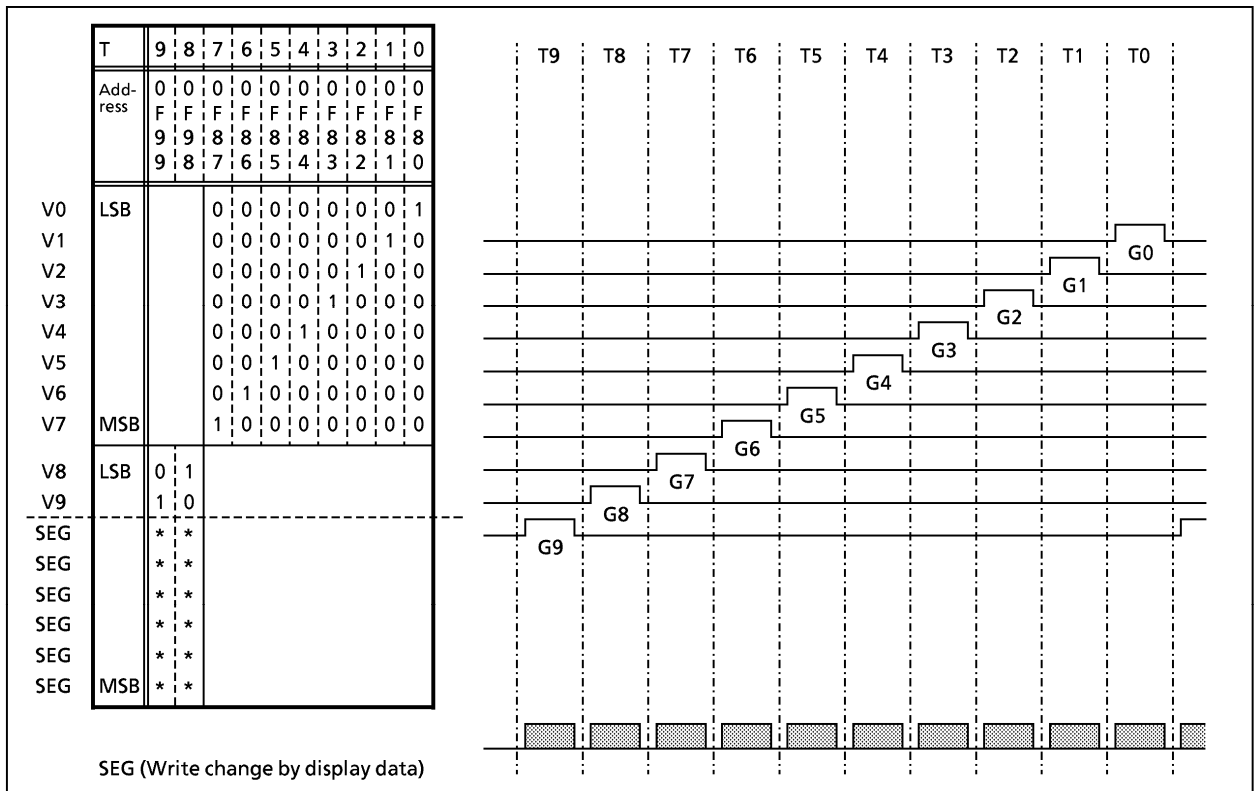
Figure 2-84. Example of Conventional type VFT driver pulse
