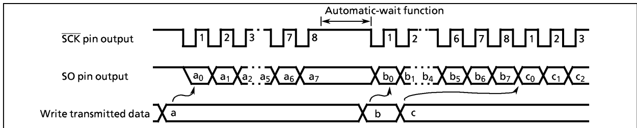
Figure 2-49. Automatic-wait Function
