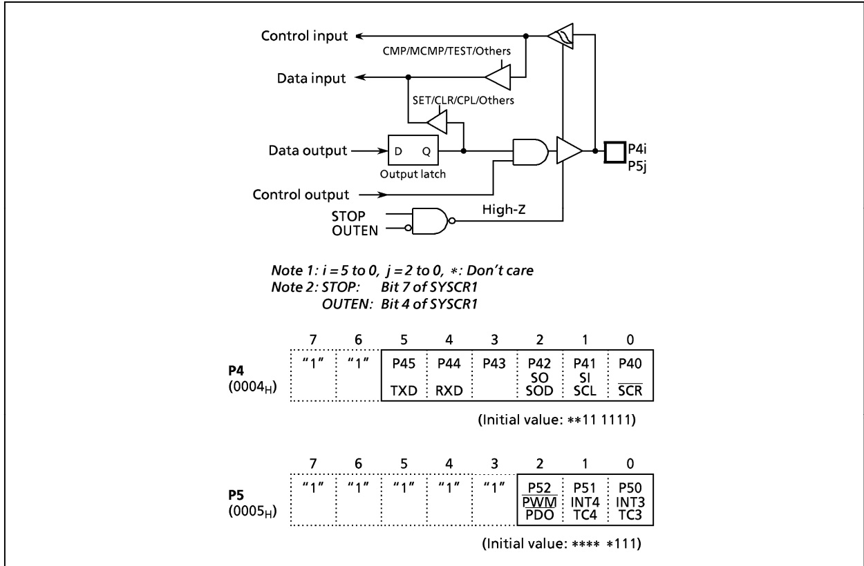
Figure 2-7. Ports P4 and P5
