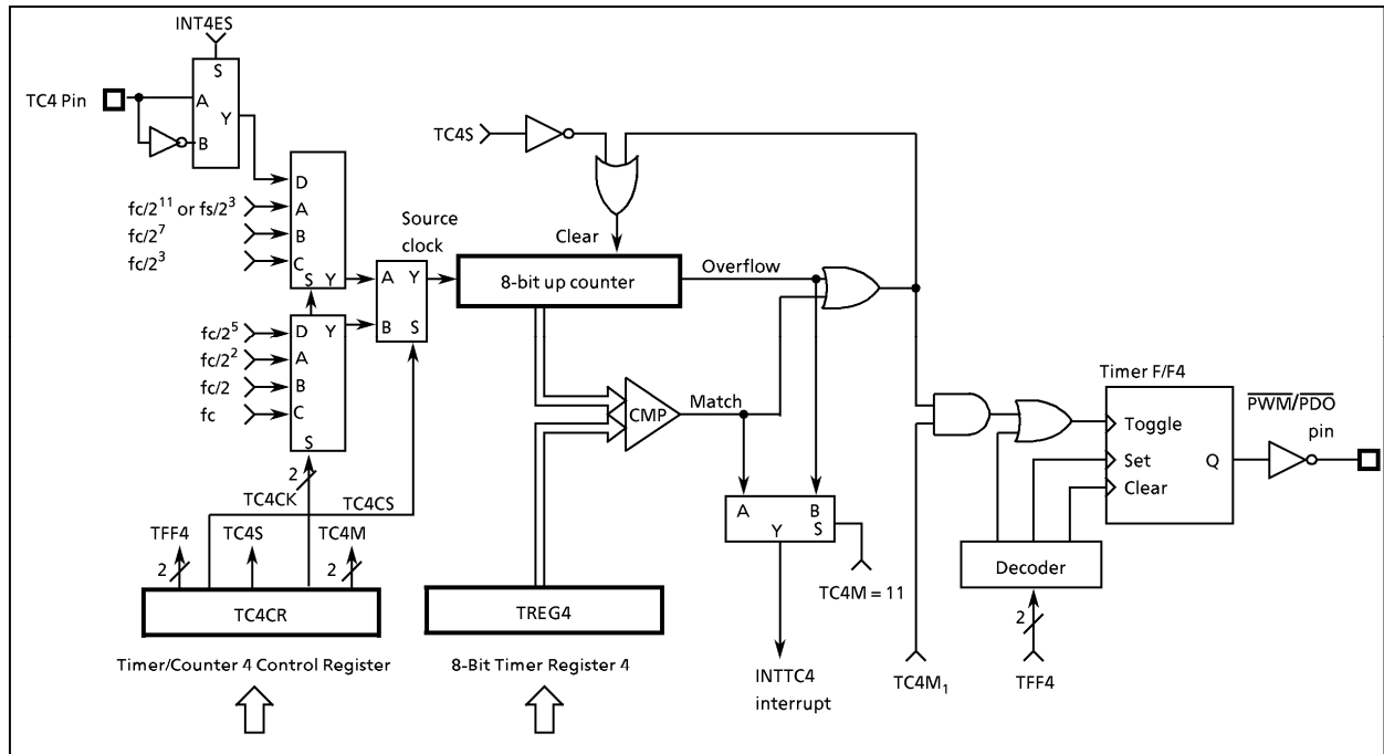
Figure 2-29. Timer/Counter 4
