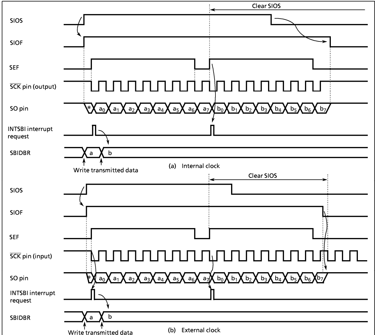
Figure 2-52. Transfer Mode
