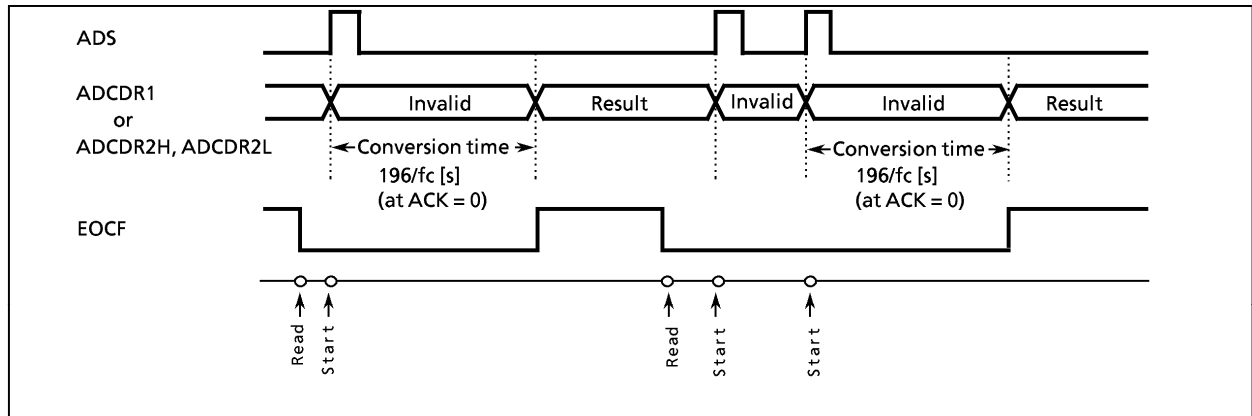
Figure 2-72. AD Conversion Timing Chart
