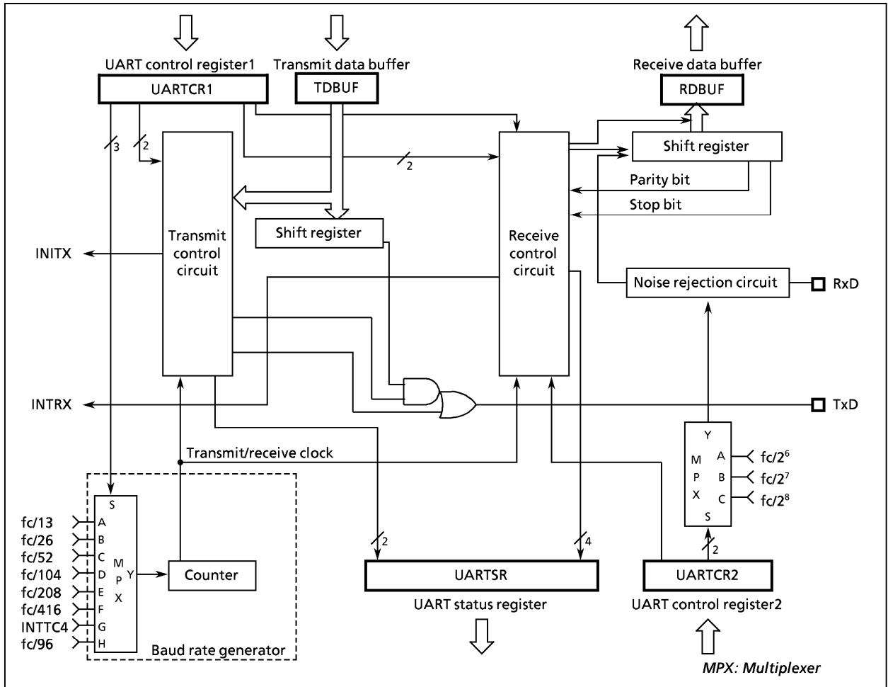
Figure 2-57. UART
