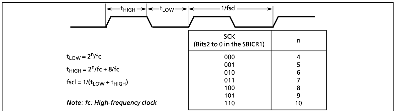
Figure 2-36. Clock Source
