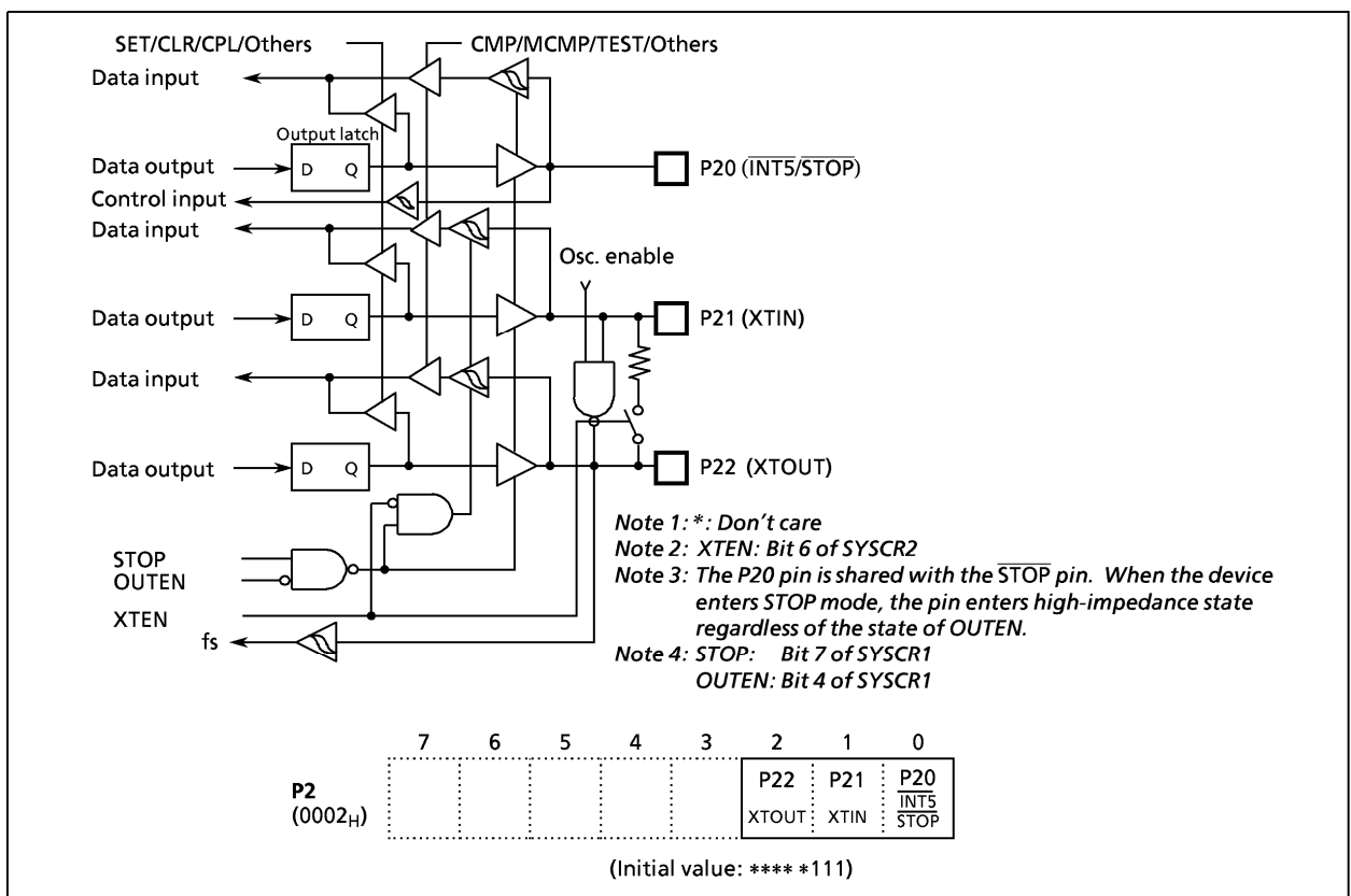
Figure 2-5 (1). Port P2
