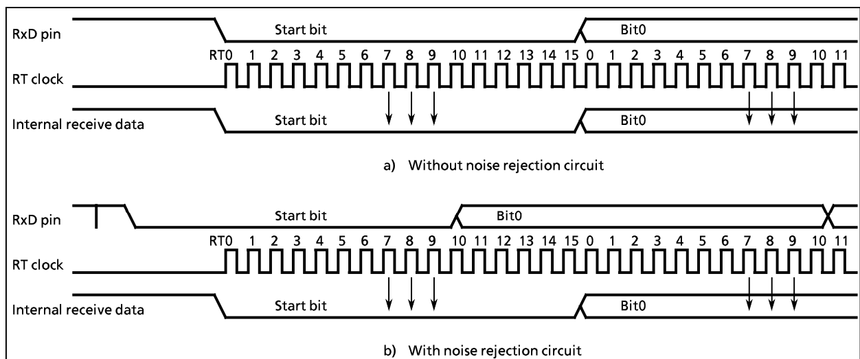
Figure 2-60. Data Sampling
