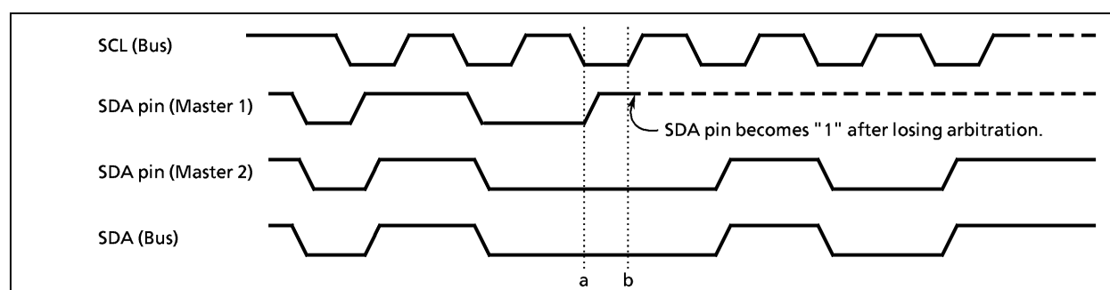
Figure 2-40. Arbitration Lost
