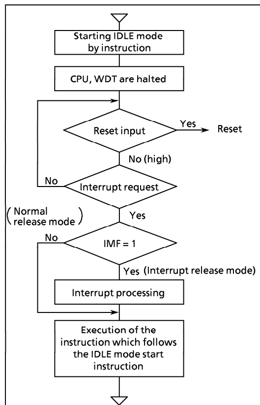
Figure 1-19. IDLE Mode
