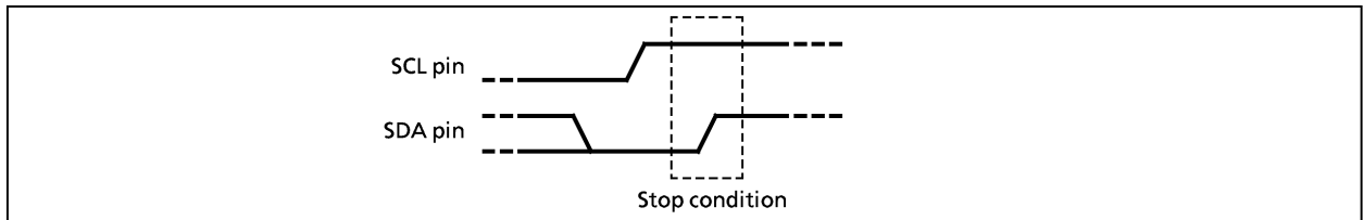
Figure 2-39. Stop Condition Generation
