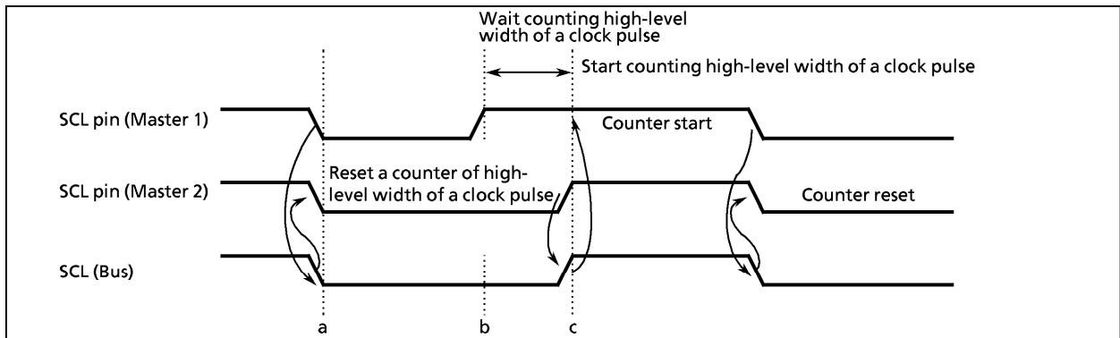
Figure 2-37. Clock Synchronization
