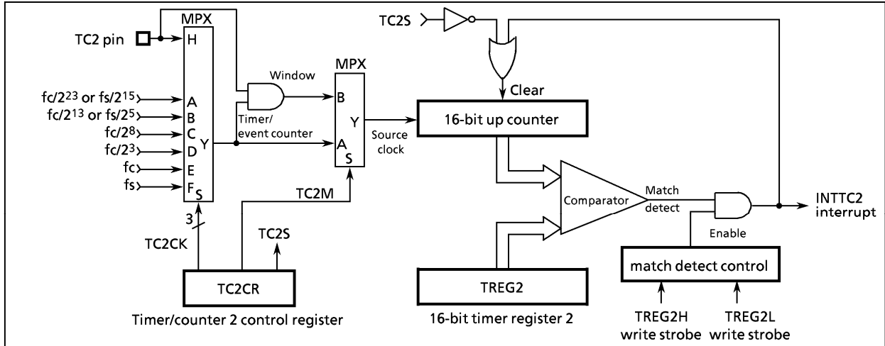
Figure 2-23. Timer/Counter 2 (TC2)
