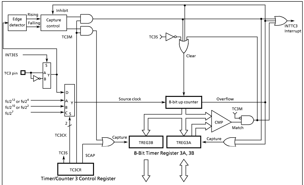
Figure 2-26. Timer/Counter 3
