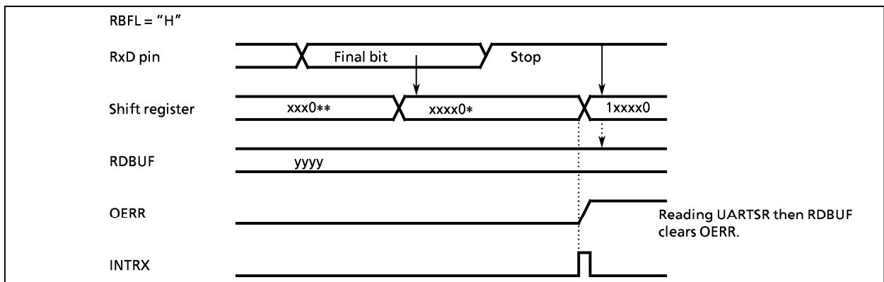
Figure 2-63. Generation of Overrun Error
