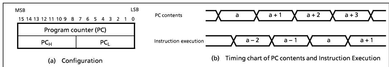
Figure 1-3. Program Counter
