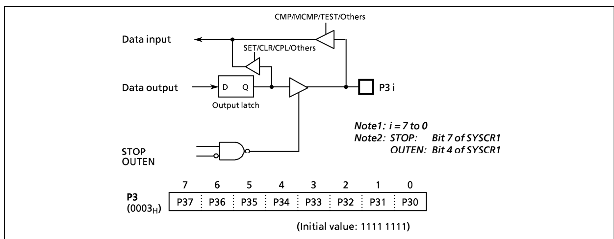
Figure 2-6. Port P3
