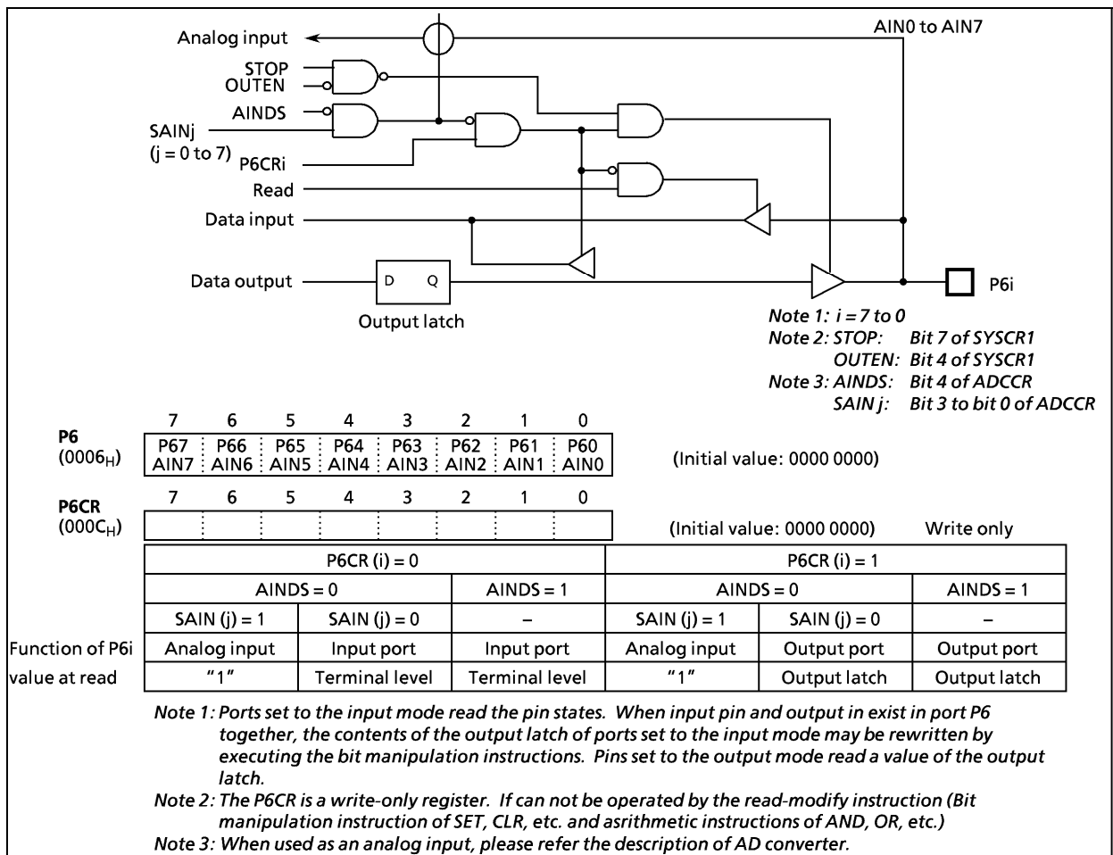
Figure 2-8. Port P6
