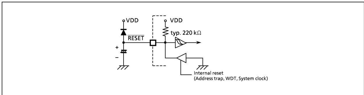
Figure 1-Figure 1-30. Simple Power-on-reset Circuitry
