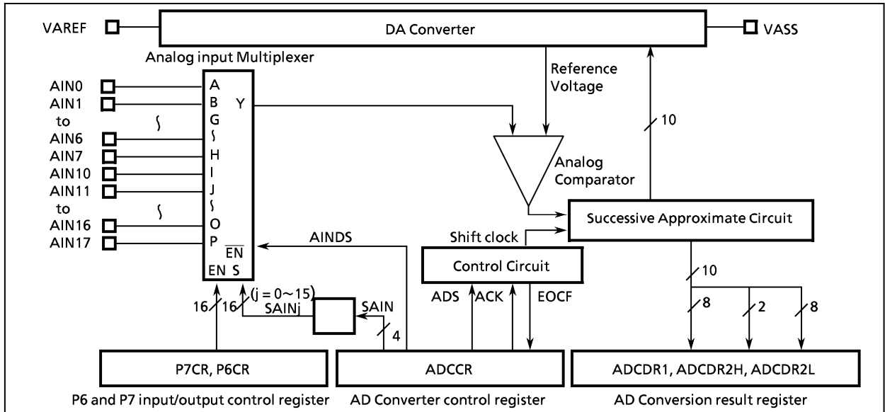
Figure 2-69. AD Converter
