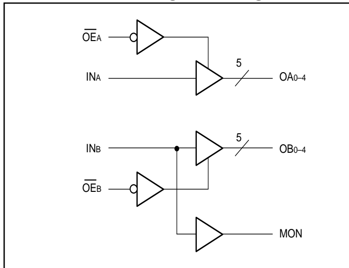
PI49FCT805T/2805T Logic Block Diagram
