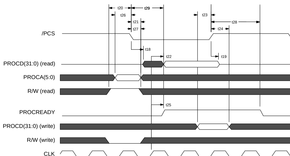
Figure 6: Processor Port Cycle
