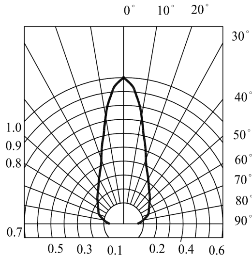
RADIATION DIAGRAM
