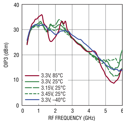
Output IP3 vs RF Frequency ( P_{LOM} = 10dBm )
