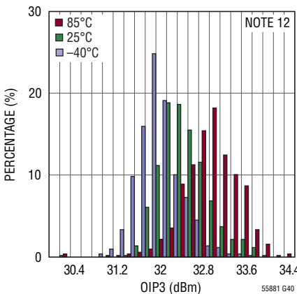
Output IP3 Distribution at 2140MHz
