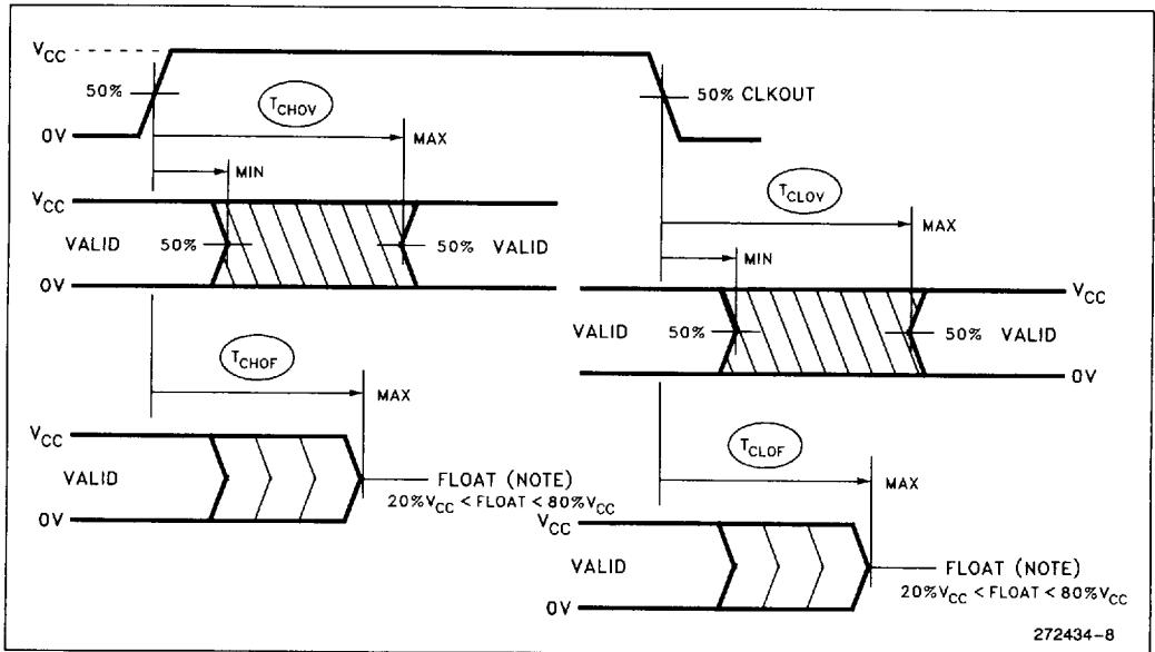
Figure 9. Output Delay and Float Waveforms
