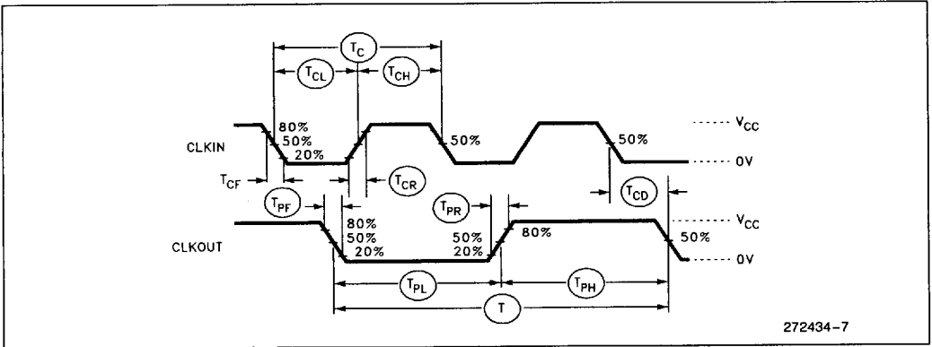
Figure 8. Input and Output Clock Waveforms
