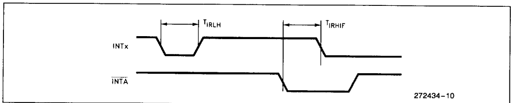
Figure 11. Relative Interrupt Signal Timings
