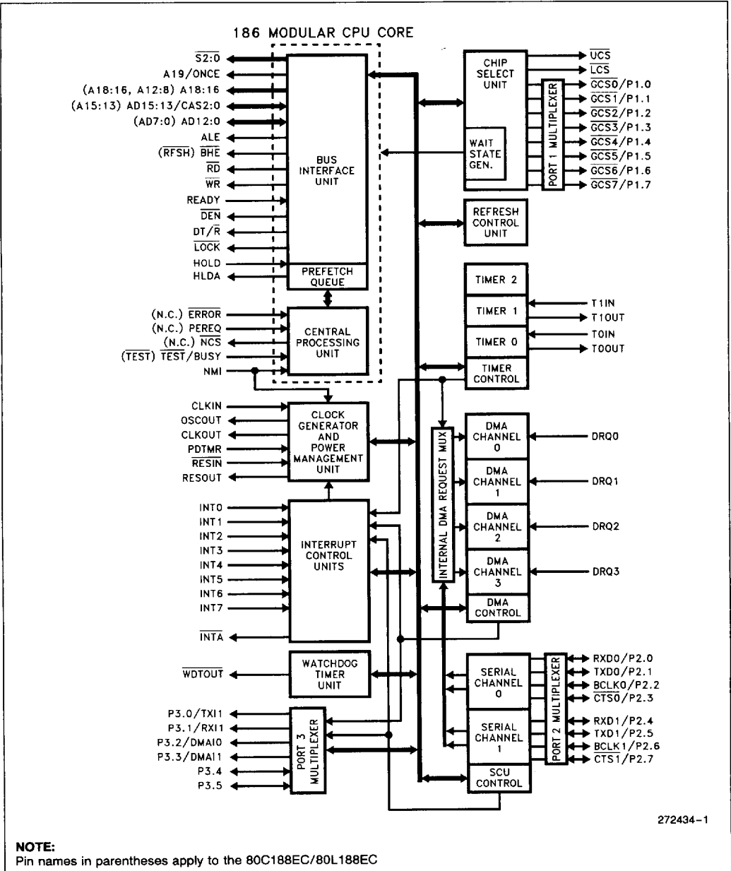
Figure 1. 80C186EC/80L186EC Block Diagram
