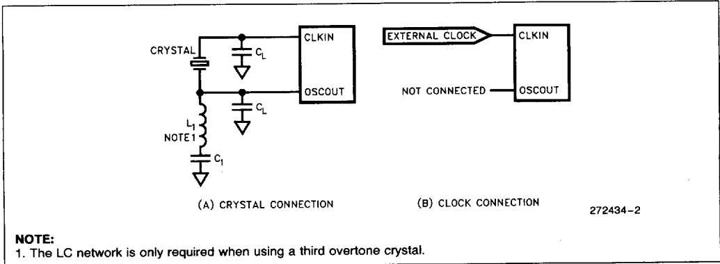
Figure 2. 80C186EC Clock Connections
