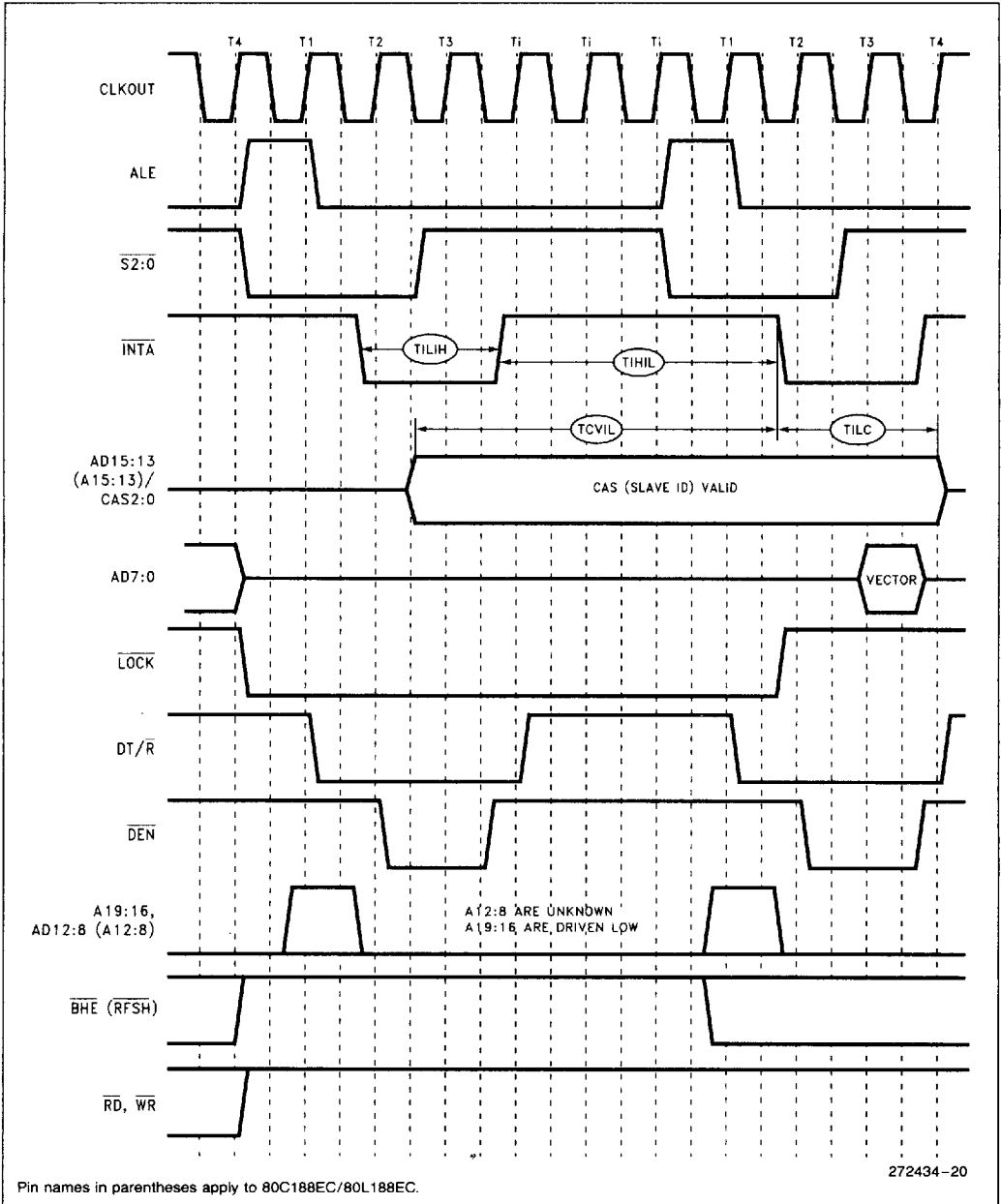
Figure 21. Interrupt Acknowledge Cycle Waveforms
