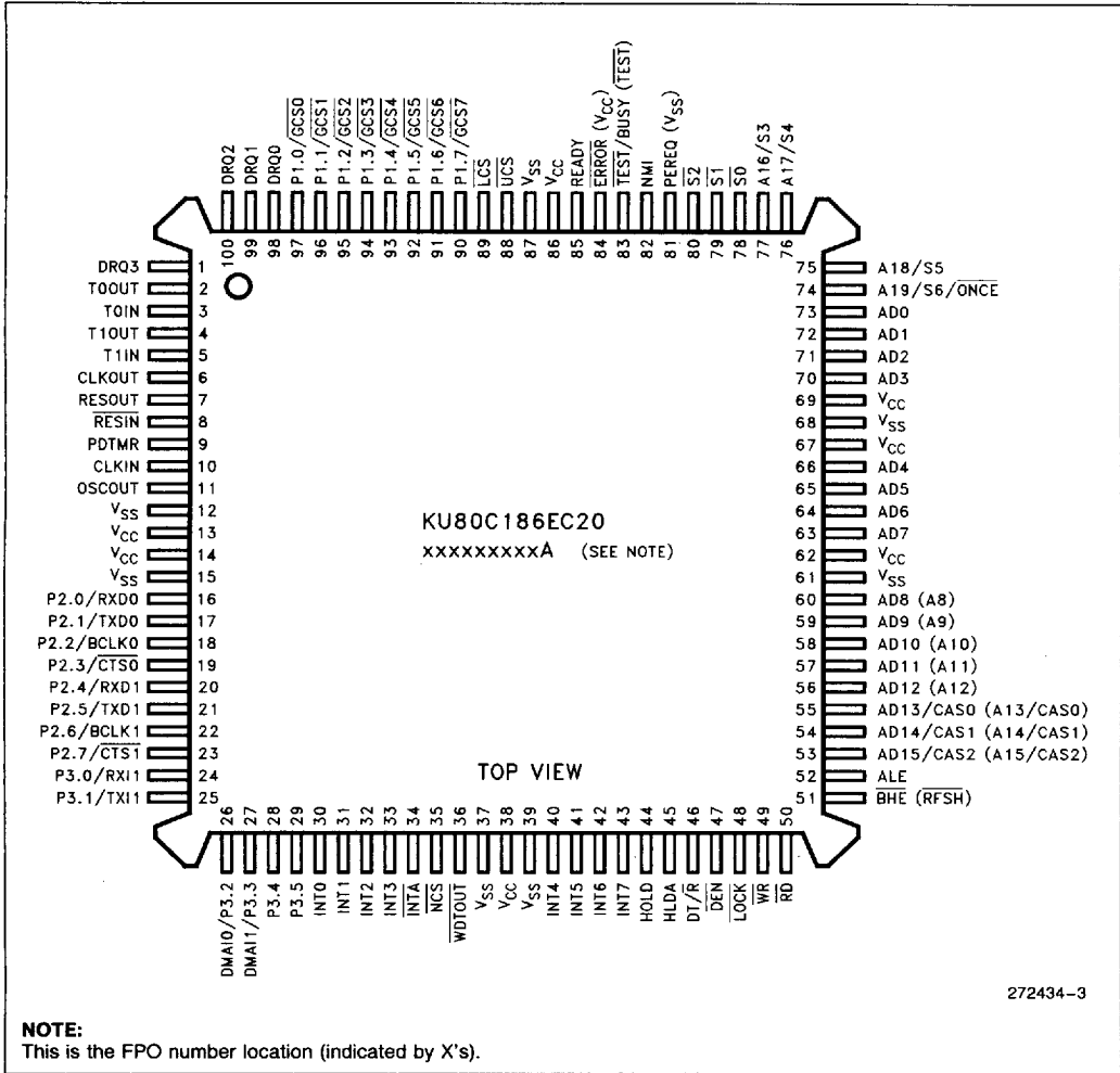
Figure 4. 100-Pin Plastic Quad Flat Pack Package (PQFP)
