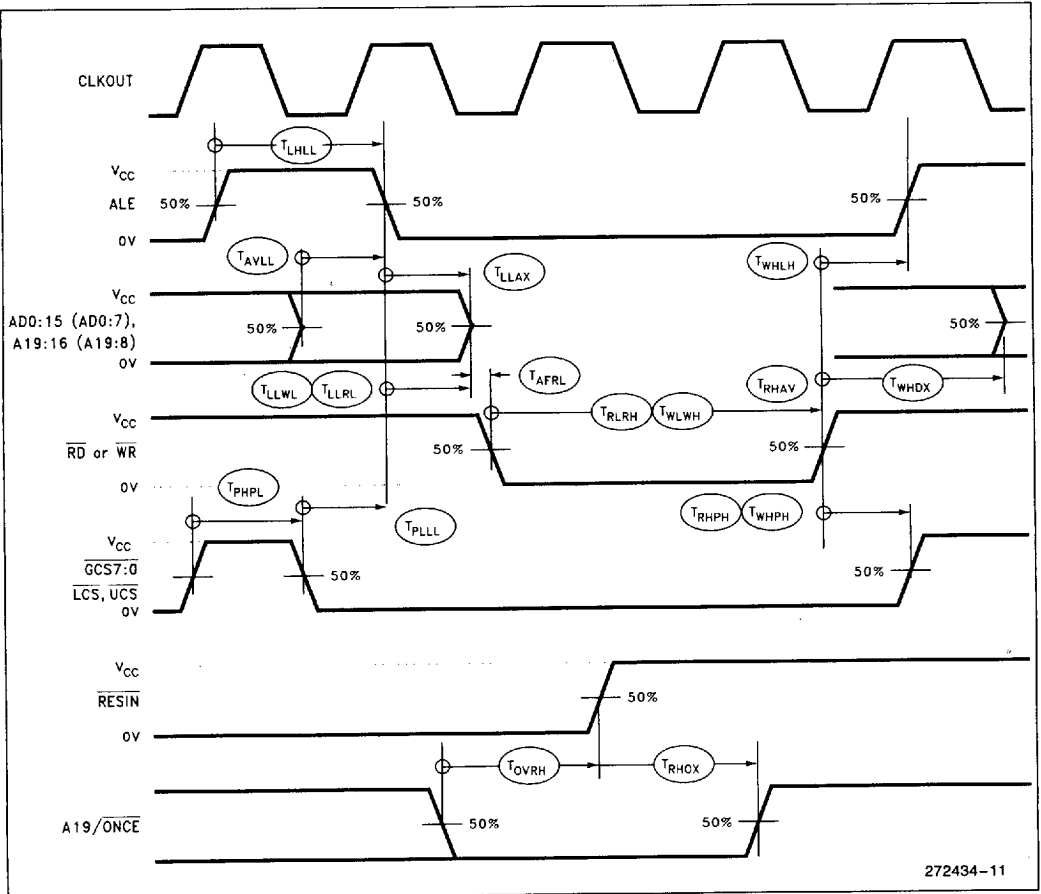
Figure 12. Relative Signal Waveform
