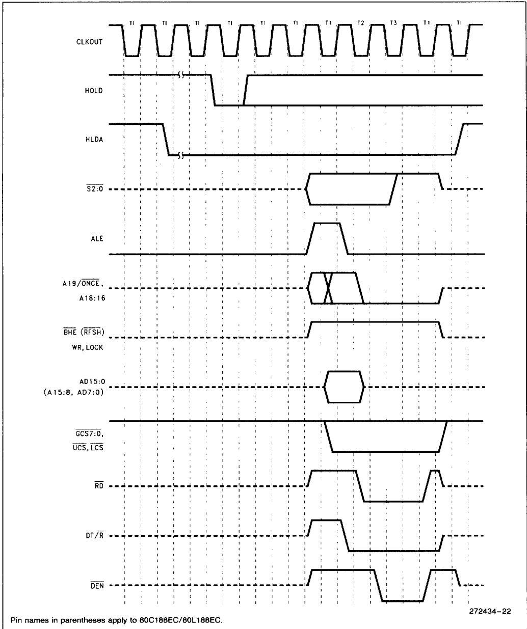
Figure 23. Refresh during HLDA Waveforms
