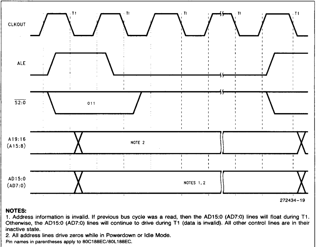
Figure 20. Halt Cycle Waveforms
