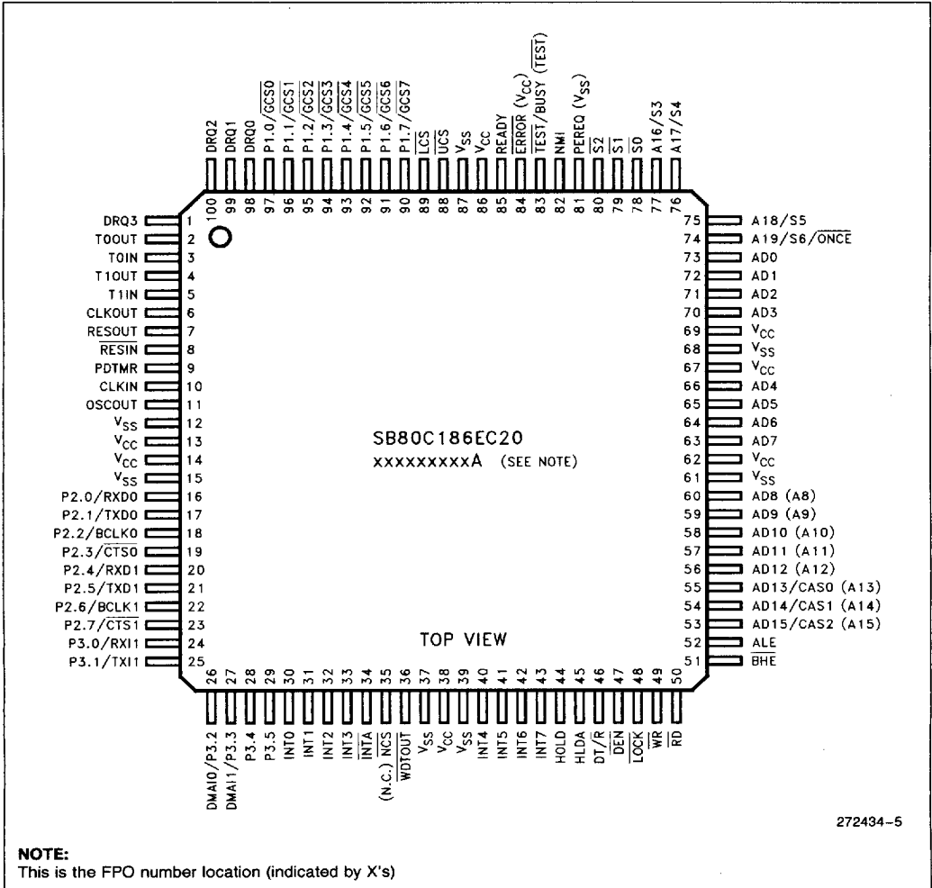
Figure 6. 100-Pin Shrink Quad Flat Pack Package (SQFP)
