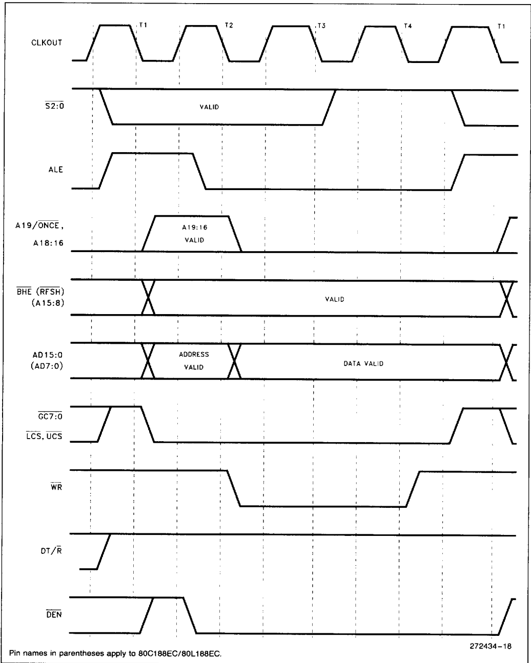
Figure 19. Memory Write and I/O Write Cycle Waveforms
