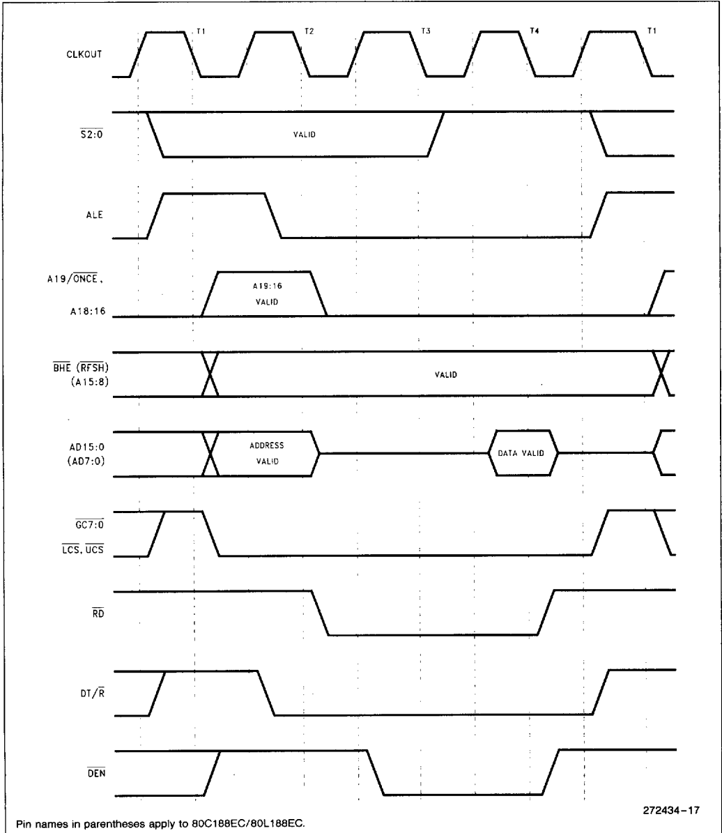
Figure 18. Memory Read, I/O Read, Instruction Fetch and Refresh Waveforms
