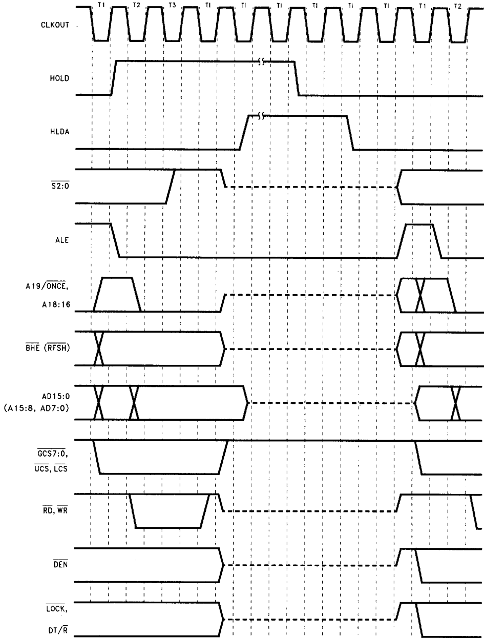
Figure 22. HOLD/HLDA Cycle Waveforms
