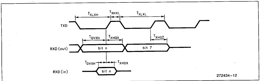
Figure 13. Serial Port Mode 0 Waveform
