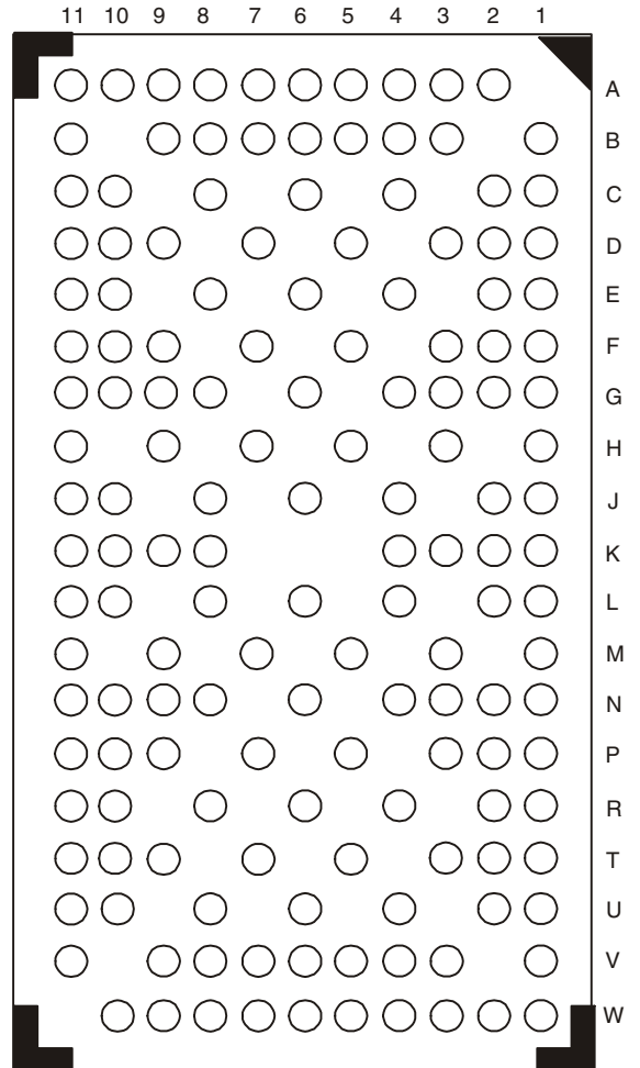
BOTTOM VIEW
