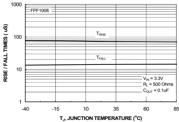
Figure 13. FPF1008 T_{RISE} / T_{FALL} vs. Temperature
