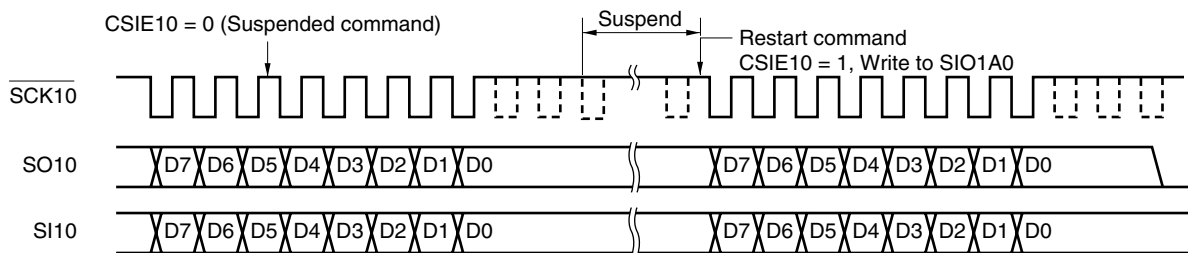
Figure 12-16. Automatic Transmission/Reception Suspension and Restart
