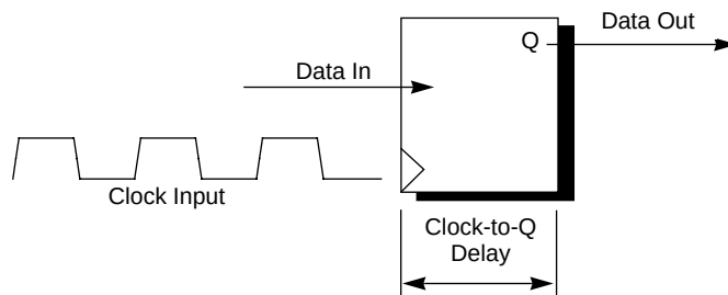
Figure 10-2 Clock-to-Q Delay
