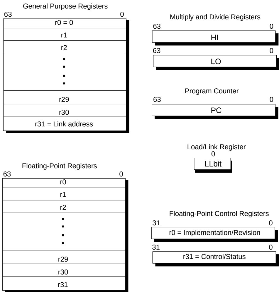
Figure 1-2 CPU Registers
