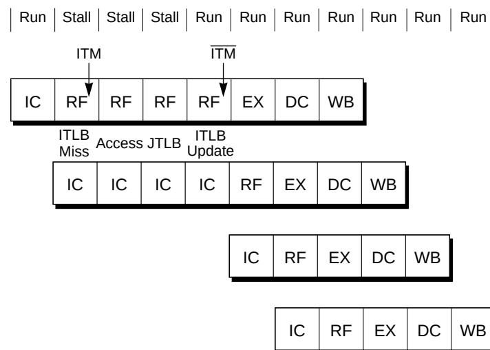
Figure 4-13 Instruction TLB Miss Interlock
