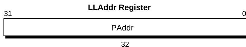
Figure 5-17 LLAddr Register
