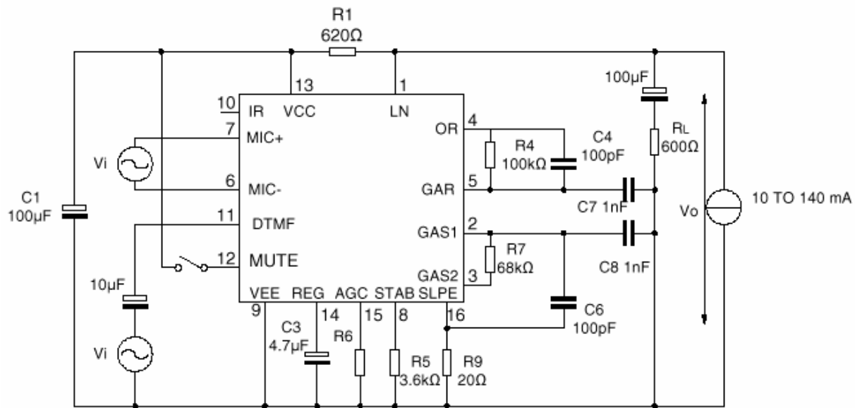
Fig.13 Test circuit defining voltage gain of MIC+, MIC- and DTMF inputs. Voltage gain is defined as: G_v=20*\log (|V_O/V_i|) . For measuring the gain from MIC+ and MIC- the MUTE input should be LOW or open-circuit, for measuring the DTMF input MUTE should be HIGH .Inputs not under test should be open-circuit.
