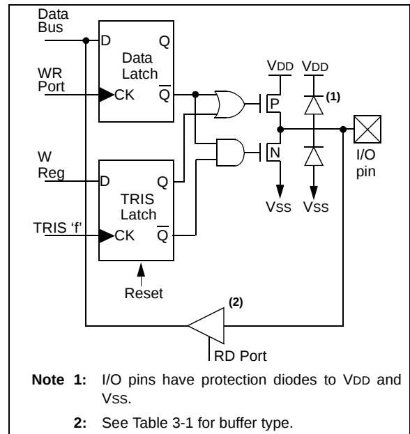
FIGURE 5-1: EQUIVALENT CIRCUIT FOR A SINGLE I/O PIN
