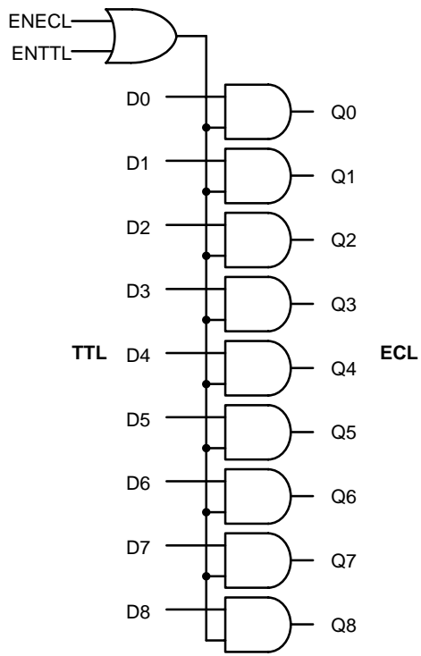
Figure 2. Logic Symbol
