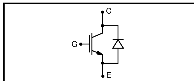
Fig.2 ITH23C06 circuit
