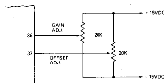
Figure 1. External Adjustment
