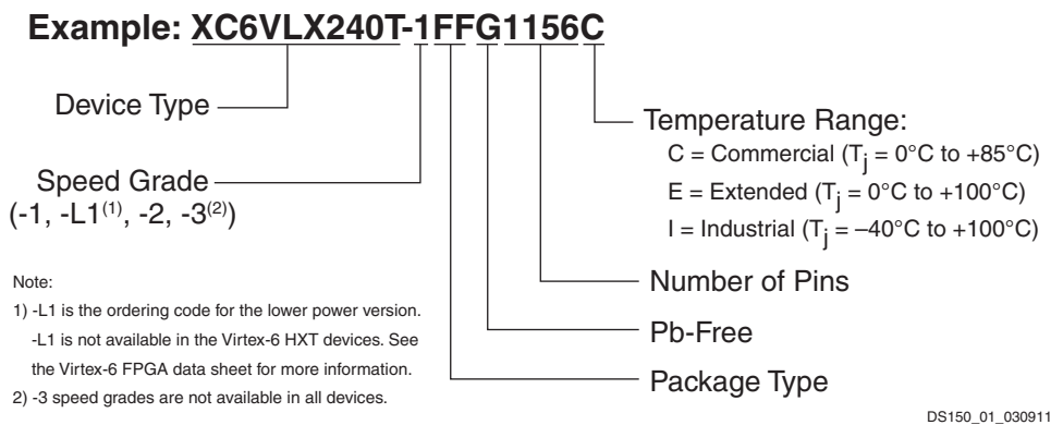
Figure 1: Virtex-6 FPGA Ordering Information
